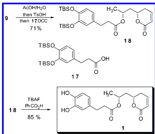
Scheme 6
