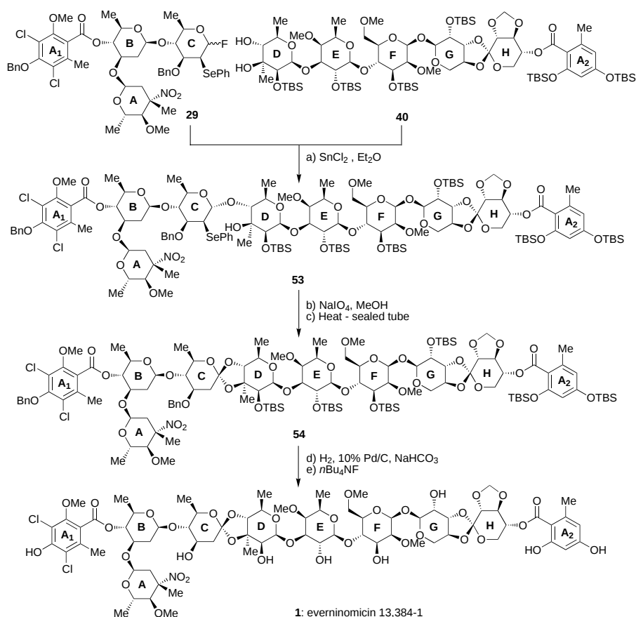
Scheme 8. Final stages of the total synthesis of everninomicin 13,384-1 ( 1 ). a) 2.4 equiv 29 , 2.0 equiv \text{SnCl}_2 , \text{Et}_2\text{O} , 0 \rightarrow 25^\circ\text{C} , 6 h, 70%; b) 10.0 equiv \text{NaIO}_4 , 8.0 equiv \text{NaHCO}_3 , \text{MeOH}/\text{CH}_2\text{Cl}_2/\text{H}_2\text{O} 3:2:1, 25^\circ\text{C} , 4 h; c) vinyl acetate/toluene/diisopropylamine 2:2:1, sealed tube, 140^\circ\text{C} , 12 h, 65% over two steps; d) \text{H}_2 , 0.2 equiv 10% \text{Pd/C} , \text{NaHCO}_3 ( w/w ), 4.0 equiv \text{NaHCO}_3 , t \text{BuOMe} , 25^\circ\text{C} , 1 h; e) 10.0 equiv n \text{Bu}_4\text{NF} , THF, 25^\circ\text{C} , 10 h, 75% for two steps.
