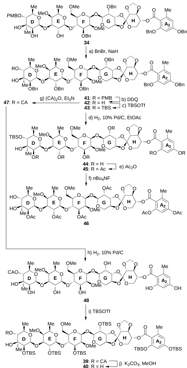
Scheme 6. Synthesis of DEFGHA 2 fragments 40 , 42 , and 46 , initial strategies. a) 3.0 equiv NaH, 2.5 equiv BnBr, 0.2 equiv nBu_4NI , DMF, 0 \rightarrow 25 ^{\circ}C , 2 h, 95 %; b) 1.5 equiv DDQ, CH_2Cl_2/H_2O 10:1, 0 \rightarrow 25 ^{\circ}C , 2 h, 95 %; c) 1.5 equiv TBSOTf, 3.0 equiv lutidine, CH_2Cl_2 , -10 \rightarrow 0 ^{\circ}C , 1 h, 96 %; d) 0.5 equiv 10 % Pd/C (w/w), EtOAc, 25 ^{\circ}C , 6 h; e) 10.0 equiv Ac_2O , 20 equiv Et_3N , 0.2 equiv 4-DMAP, CH_2Cl_2 , 0 \rightarrow 25 ^{\circ}C , 2 h, 88 % over two steps; f) 1.5 equiv nBu_4NF , 1.5 equiv AcOH, THF, 0 \rightarrow 25 ^{\circ}C , 2 h, 90 %; g) 1.5 equiv (CA)_2O , 3.0 equiv Et_3N , 0.2 equiv 4-DMAP, CH_2Cl_2 , 0 \rightarrow 25 ^{\circ}C , 1 h, 98 %; h) 0.5 equiv 10 % Pd/C (w/w), EtOAc, 25 ^{\circ}C , 4 h; i) 8.0 equiv TBSOTf, 20 equiv 2,6-di- tert -butylpyridine, CH_2Cl_2 , 0 \rightarrow 25 ^{\circ}C , 8 h, 65 % over two steps; j) 0.2 equiv K_2CO_3 , MeOH, 25 ^{\circ}C , 15 min, 85 %.
