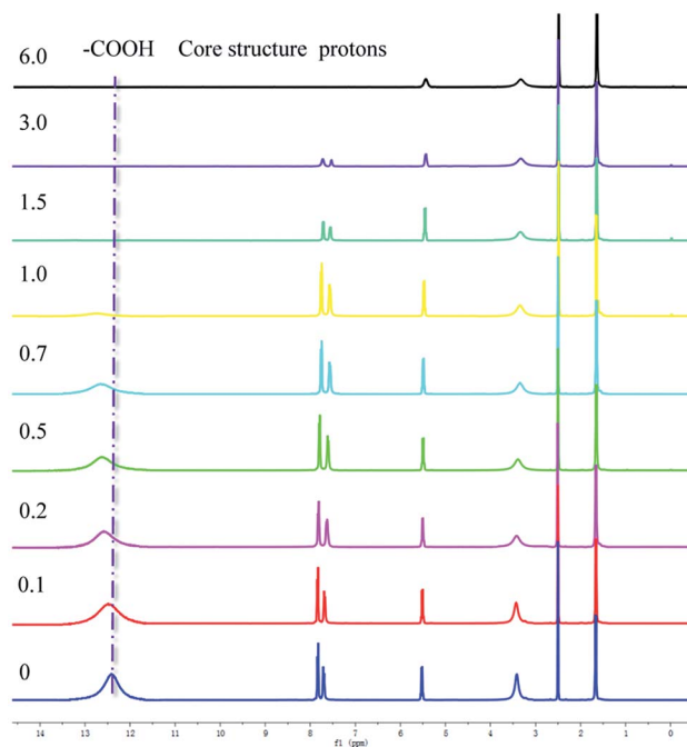
Fig. 5 The ^1H NMR titrations of H_2PDIAA with TBAF in DMSO-d_6 .
