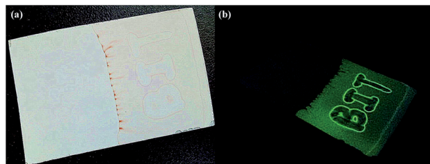
Fig. 4 Photographs of test-paper of H_2PDIAA solution in DMF ( 1 \times 10^{-5} M) of TBAF. (a) Visible light of the test-paper, (b) UV light ( \lambda = 365 nm) of the test-paper.
