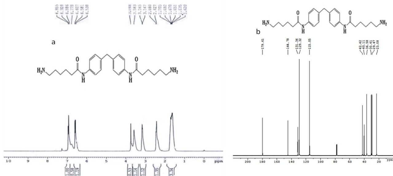
Figure 3. (a) ^1\text{H} NMR and (b) ^{13}\text{C} NMR spectra of CPA.
