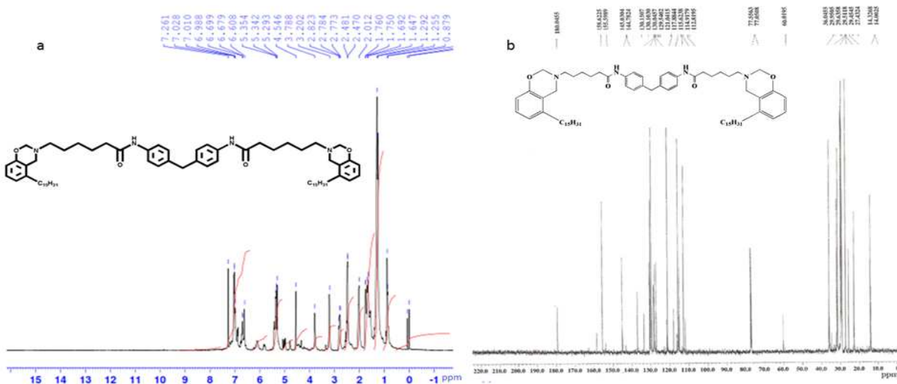
Figure 4. (a) ^1\text{H} NMR and (b) ^{13}\text{C} NMR spectra of CBZ.
