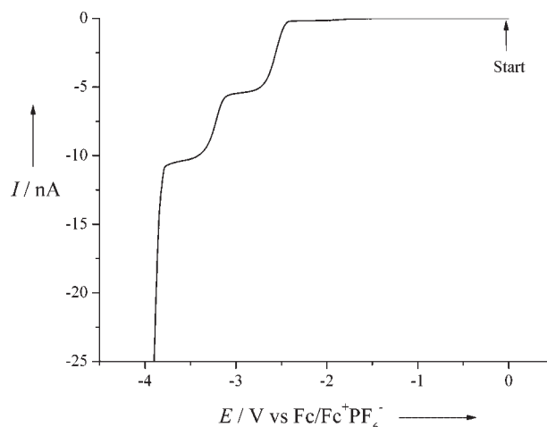
Figure 2. Voltammetric response of anthracene (3 mM) in THF (0.1 M TBAP) using a 12.5\text{ }\mu\text{m} (radius) platinum microelectrode recorded at a scan rate of 10\text{ mVs}^{-1} (at -78^{\circ}\text{C} )
