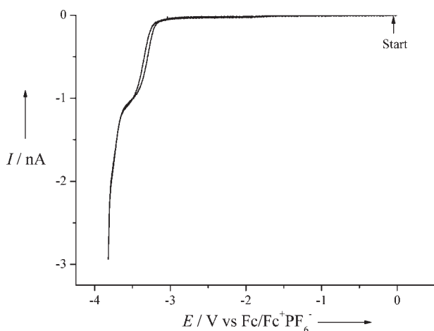
Figure 1. Voltammetric response of DBB (2.1 mM) in THF (0.1 M TBAP) using a 13\text{ }\mu\text{m} (radius) platinum microelectrode recorded at a scan rate of 10\text{ mVs}^{-1} (at -78^{\circ}\text{C} )
