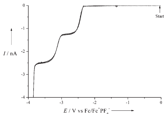
Figure 3. Voltammetric response of methyl naphthalene-1-carboxylate (3.3 mM) in THF (0.1 M TBAP) using a 5\text{ }\mu\text{m} (radius) platinum microelectrode recorded at a scan rate of 10\text{ mVs}^{-1} (at -78^{\circ}\text{C} )
