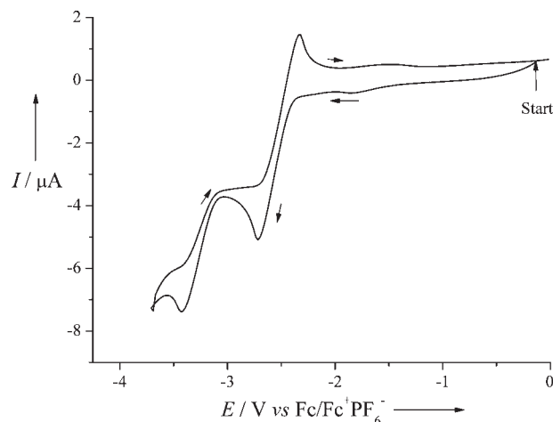
Figure 6. Cyclic voltammetry of anthracene (2.5 mM), at -78^{\circ}\text{C} in THF (0.1 M TBAP) using a platinum electrode (1 mm) recorded at a scan rate of 250\text{ mV s}^{-1}
