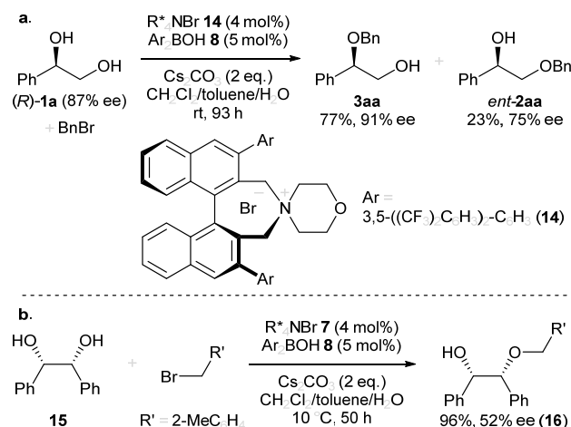
Scheme 2. a) Catalyst-controlled, regioselective alkylation of the secondary alcohol of (R)-1a. b) Desymmetrization of meso-diol 15.
