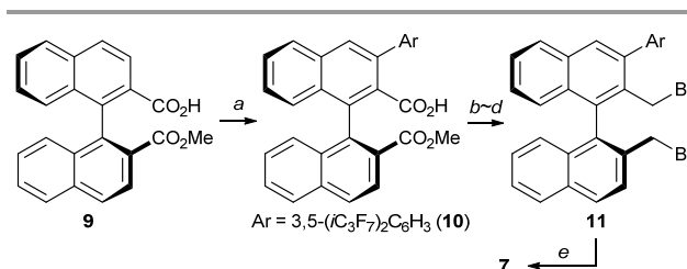
Scheme 1 Preparation of catalyst 7 . Conditions: a) [( p -cym)RuCl 2 ] 2 , Bu 3 P, 3,5-(iC 3 F 7 ) 2 C 6 H 3 , K 2 CO 3 , NMP, 110 °C, 78% yield; b) LiOH aq., THF, reflux; c) BH 3 ·Me 2 S, THF, reflux, 86% yield (2 steps); d) PBr 3 , THF, rt, 88% yield; e) NH 3 aq., CH 3 CN, 80 °C, 69% yield.
