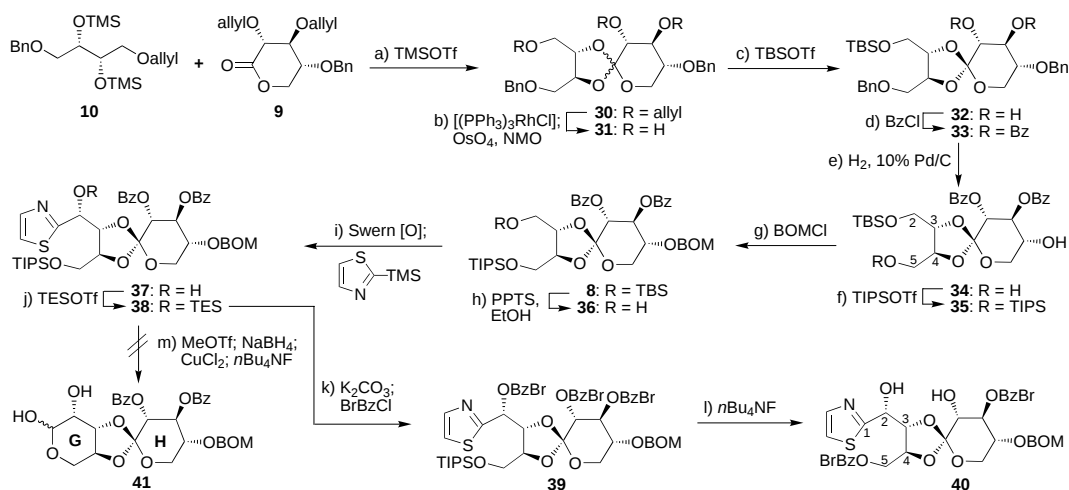
Scheme 4. Attempted assembly of GH fragment 41 . a) 2.0 equiv 10 , 1.0 equiv 9 , 0.15 equiv TMSOTf, CH 2 Cl 2 , 0 → 25 °C, 12 h, 97%, 1:1 mixture of diastereoisomers; b) i) 4.5 equiv DABCO, 0.07 equiv [(Ph 3 P) 3 RhCl], EtOH/H 2 O 10:1, reflux, 2 h; ii) 4.5 equiv NMO, 0.2 equiv OsO 4 , Me 2 CO/H 2 O 10:1, 25 °C, 8 h, 97% (two diastereoisomers ca. 1:1 ratio, more polar one shown here); c) 1.1 equiv TBSOTf, 1.5 equiv 2,6-lutidine, CH 2 Cl 2 , –78 °C, 0.5 h, 92%; d) 2.5 equiv BzCl, 4.0 equiv Et 3 N, 0.2 equiv 4-DMAP, CH 2 Cl 2 , 0 → 25 °C, 2 h, 97%; e) H 2 , 10% Pd/C 0.1 equiv w/w, EtOAc, 25 °C, 2 h, 95%; f) 1.1 equiv TIPSOTf, 1.5 equiv 2,6-lutidine, CH 2 Cl 2 , –78 °C, 0.5 h, 89%; g) 5.0 equiv BOMCl, 10.0 equiv i Pr 2 NEt, CH 2 Cl 2 , 50 °C, 4 h, 89%; h) 0.1 equiv PPTS, EtOH/THF (3:1), 50 °C, 6 h, 83%; i) i) 1.8 equiv (COCl) 2 , 2.0 equiv DMSO, –78 °C, 2 h; ii) 4.0 equiv Et 3 N, –78 → –40 °C, 2 h; iii) 2.0 equiv TMS-thiazole, –40 → 25 °C, 12 h; iv) 0.06 equiv PPTS, MeOH, 25 °C, 2 h, 97%, ca. 10:1 mixture of diastereoisomers; j) 1.1 equiv TESOTf, 1.2 equiv 2,6-lutidine, CH 2 Cl 2 , 0 °C, 0.5 h, 89%; k) 0.5 equiv K 2 CO 3 , MeOH, 25 °C, 1 h; 4.0 equiv BrBzCl, 5.0 equiv Et 3 N, 0.2 equiv 4-DMAP, CH 2 Cl 2 , 0 → 25 °C, 2 h, 86% over two steps; l) 1.3 equiv n Bu 4 NF, THF, 25 °C, 1 h, 88%; m) i) 1.2 equiv MeOTf, MeCN, 25 °C, 0.5 h; ii) 2.4 equiv NaBH 4 , MeOH, 0 → 25 °C, 0.5 h; iii) 1.2 equiv CuCl 2 , 8.0 equiv CuO, MeCN/H 2 O 5:1, 25 °C, 2 h; iv) 2.5 equiv n Bu 4 NF, THF, 25 °C, 2 h, decomposition. DABCO = 1,4-diazabicyclo[2.2.2]octane; NMO = N -methylmorpholine N -oxide; PPTS = pyridinium p -toluenesulfonate; BrBz = p -bromobenzoate, TES = triethylsilyl; THF = tetrahydrofuran.
