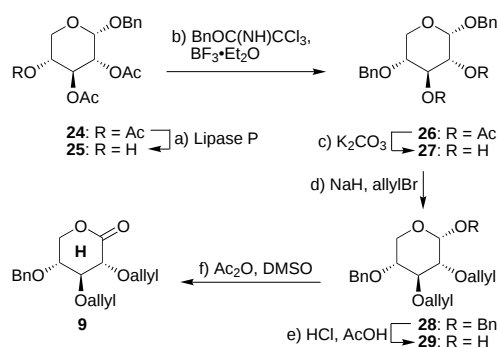
Scheme 3. Synthesis of carbohydrate building block H ( 9 ). a) 2.0 equiv Lipase P ( w/w ), 2.0 equiv isoamyl alcohol, isooctane, 25 °C, 96 h, 84 %; b) 0.1 equiv BF 3 ·Et 2 O, 1.2 equiv BnOC(NH)CCl 3 , CH 2 Cl 2 , 0 °C, 3 h, 91 %; c) 0.2 equiv K 2 CO 3 , MeOH/Et 2 O 1:1, 25 °C, 1 h, 97 %; d) 2.2 equiv NaH, 3.2 equiv allyl bromide, DMF, 0 → 25 °C, 2 h, 92 %; e) 1N HCl in AcOH 1:40, 80 °C, 5 h, 91 %; f) Ac 2 O/DMSO (1:2), 25 °C, 12 h, 96 %. DMSO = dimethyl sulfoxide.
