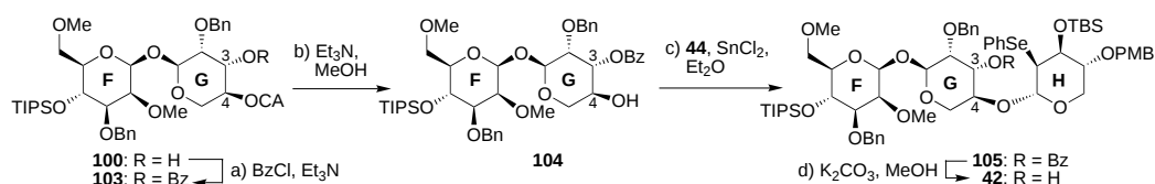
Scheme 12. Recycling of FG fragment 100 and synthesis of FGH fragment 42 . a) 1.2 equiv \text{BzCl} , 2.0 equiv \text{Et}_3\text{N} , 0.2 equiv 4-DMAP, \text{CH}_2\text{Cl}_2 , 0 \rightarrow 25 °C, 2 h, 96 %; b) 2.0 equiv \text{Et}_3\text{N} , MeOH/ \text{CH}_2\text{Cl}_2 1:1, 40 °C, 6 h, 96 %; c) 2.0 equiv 44 , 1.8 equiv \text{SnCl}_2 , 0 \rightarrow 25 °C, \text{Et}_2\text{O} , 3 h, 92 %; d) 0.2 equiv \text{K}_2\text{CO}_3 , MeOH/ \text{Et}_2\text{O} 1:1, 25 °C, 12 h, 98 %.
