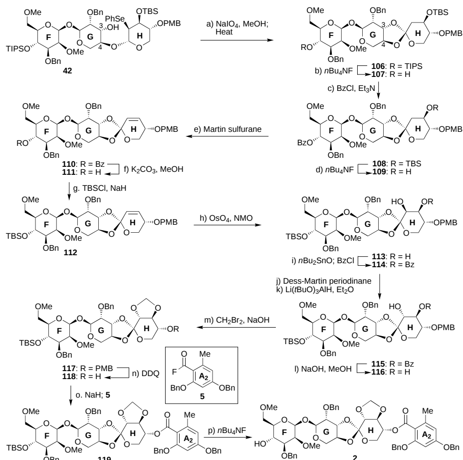
Scheme 13. Completion of the synthesis of the FGHA 2 fragment 2 . a) i) 10.0 equiv \text{NaIO}_4 , 8.0 equiv \text{NaHCO}_3 , MeOH/ \text{CH}_2\text{Cl}_2 / \text{H}_2\text{O} 3:2:1, 25 °C, 2 h; ii) vinyl acetate/toluene/diisopropylamine 2:2:1, sealed tube, 140 °C, 12 h, 81 % over two steps; b) 1.1 equiv n\text{Bu}_4\text{NF} , THF, 0 °C, 0.5 h, 95 %; c) 1.2 equiv \text{BzCl} , 1.8 equiv \text{Et}_3\text{N} , 0.2 equiv 4-DMAP, \text{CH}_2\text{Cl}_2 , 0 \rightarrow 25 °C, 2 h, 97 %; d) 1.5 equiv n\text{Bu}_4\text{NF} , 0.2 equiv AcOH, THF, 25 °C, 1 h, 95 %; e) 4.0 equiv Martin sulfurane, 0.05 equiv \text{Et}_3\text{N} , \text{CHCl}_3 , 50 °C, 2 h, 85 %; f) 0.5 equiv \text{K}_2\text{CO}_3 , MeOH, 25 °C, 6 h, 90 %; g) 6.0 equiv NaH, 12 equiv TBSCl, 1.0 equiv [18]crown-6, THF, 0 °C, 2 h, 80 %; h) 5.0 equiv NMO, 0.5 equiv \text{OsO}_4 , 1.0 equiv quinuclidine, \text{Me}_2\text{CO}/\text{H}_2\text{O} 10:1, 25 °C, 36 h, 70 %, 8:1 mixture of diastereoisomers; i) 1.1 equiv n\text{Bu}_2\text{SnO} , MeOH, reflux, 3 h; 1.5 equiv \text{BzCl} , 1,4-dioxane, 15 °C, 0.5 h, 97 %, 5:1 mixture of regioisomers; j) 2.0 equiv Dess–Martin periodinane, 20 equiv \text{NaHCO}_3 , \text{CH}_2\text{Cl}_2 , 25 °C, 1 h; k) 1.1 equiv \text{Li}(\text{tBuO})_3\text{AlH} , \text{Et}_2\text{O} , –10 °C, 1 h, 80 % over two steps; l) 0.5 equiv NaOH, MeOH, 25 °C, 1 h, 98 %; m) 3.0 equiv n\text{Bu}_4\text{NBr} , \text{CH}_2\text{Br}_2 :50 % aqueous NaOH 1:1, 65 °C, 2 h, 90 %; n) 1.5 equiv DDQ, \text{CH}_2\text{Cl}_2 / \text{H}_2\text{O} 10:1 (pH 7) 0 \rightarrow 25 °C, 1 h, 85 %; o) 1.2 equiv NaH, THF, 0 °C; then 1.5 equiv 5 , 0 \rightarrow 25 °C, 2 h, 96 %; p) 1.2 equiv n\text{Bu}_4\text{NF} , THF, 25 °C, 1 h, 91 %.
