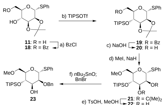
Scheme 2. Attempted synthesis of carbohydrate building block F ( 6 ). a) 1.0 equiv BzCl, 1.2 equiv Et 3 N, 0.1 equiv 4-DMAP, CH 2 Cl 2 , 0 → 25 °C, 2 h, 91 %; b) 1.2 equiv TIPSOTf, 1.4 equiv 2,6-lutidine, CH 2 Cl 2 , 0 → 25 °C, 3 h, 99 %; c) 0.2 equiv NaOH, MeOH/Et 2 O 1:1, 25 °C, 1 h, 94 %; d) 1.2 equiv NaH, 1.6 equiv MeI, DMF, 0 → 25 °C, 2 h, 92 %; e) 0.03 equiv TsOH, 1.2 equiv (CH 2 OH) 2 , MeOH/Et 2 O 10:1, 25 °C, 8 h, 87 % based on 62 % conversion; f) 1.1 equiv n Bu 4 SnO, toluene, reflux, 3 h; 1.2 equiv BnBr, 0.2 equiv n Bu 4 NI, 25 → 110 °C, 5 h, 81 %. Ts = p -toluenesulfonyl; 4-DMAP = 4-dimethylaminopyridine; DMF = dimethylformamide.
