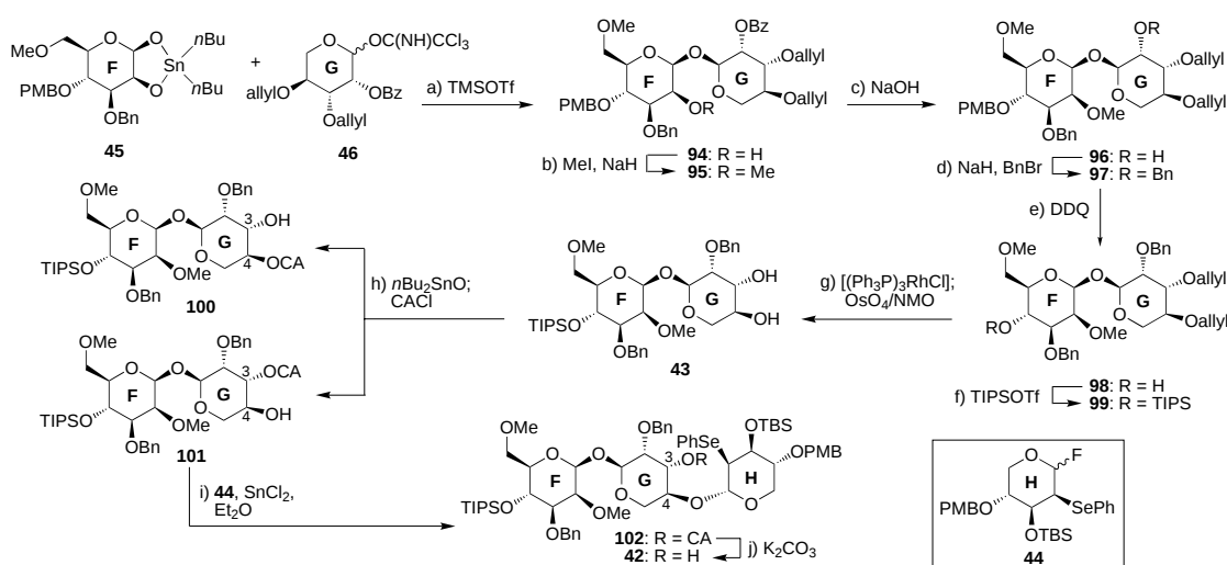
Scheme 11. Assembly of FGHA 2 fragment. a) 1) 2.1 equiv 45 , 1.0 equiv 46 , 0.5 equiv TMSOTf, \text{CH}_2\text{Cl}_2 , 0 \rightarrow 25^\circ\text{C} , 12 h; 2) 0.3 equiv PPTS, \text{MeOH} , 25^\circ\text{C} , 1 h, 74% over two steps; b) 1.1 equiv \text{NaH} , 3.0 equiv \text{MeI} , \text{DMF} , 0 \rightarrow 25^\circ\text{C} , 1 h, 87%; c) 0.3 equiv \text{NaOH} , \text{MeOH}/\text{Et}_2\text{O} 1:1, 25^\circ\text{C} , 1 h, 95%; d) 1.1 equiv \text{NaH} , 1.3 equiv \text{BnBr} , 0.2 equiv n\text{Bu}_4\text{NI} , \text{DMF} , 0 \rightarrow 25^\circ\text{C} , 4 h, 90%; e) 1.5 equiv DDQ, \text{CH}_2\text{Cl}_2/\text{H}_2\text{O} 10:1, 0 \rightarrow 25^\circ\text{C} , 1 h, 91%; f) 1.2 equiv TIPSOTf, 1.5 equiv 2,6-lutidine, \text{CH}_2\text{Cl}_2 , 0 \rightarrow 25^\circ\text{C} , 1 h, 97%; g) 1) 2.5 equiv DABCO, 0.1 equiv [(\text{Ph}_3\text{P})_3\text{RhCl}] , \text{EtOH}/\text{H}_2\text{O} 10:1, reflux, 2 h; 2) 2.2 equiv NMO, 0.05 equiv \text{OsO}_4 , \text{Me}_2\text{CO}/\text{H}_2\text{O} 10:1, 25^\circ\text{C} , 8 h, 81% over two steps; h) 1.1 equiv n\text{Bu}_4\text{SnO} , toluene, reflux, 3 h; 1.05 equiv \text{CACl} , 0 \rightarrow 25^\circ\text{C} , 1 h, 97%; 1:1 mixture of regioisomers; i) 2.0 equiv 44 , 1.8 equiv \text{SnCl}_2 , 0 \rightarrow 25^\circ\text{C} , \text{Et}_2\text{O} , 3 h, 92%; j) 0.2 equiv \text{K}_2\text{CO}_3 , \text{MeOH}/\text{Et}_2\text{O} 1:1, 25^\circ\text{C} , 1 h, 98%. CA = chloroacetyl; DDQ = 2,3-dichloro-5,6-dicyano-1,4-benzoquinone.
