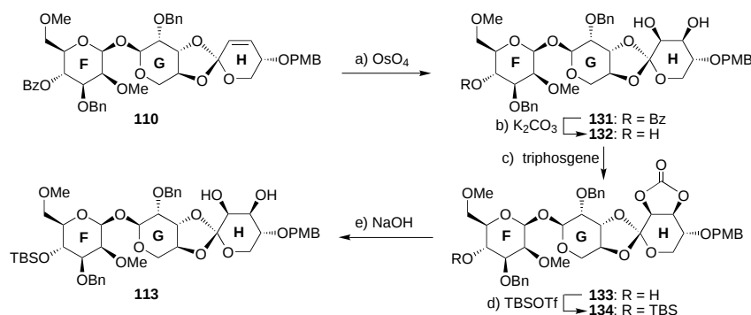
Scheme 16. Alternative synthesis of FGH fragment 113 . a) 5.0 equiv NMO, 0.5 equiv \text{OsO}_4 , 1.0 equiv quinuclidine, \text{Me}_2\text{CO}/\text{H}_2\text{O} 10:1, 25^\circ\text{C} , 24 h, 97% based on 70% conversion, 10:1 mixture of diastereoisomers; b) 0.2 equiv \text{K}_2\text{CO}_3 , \text{MeOH} , 25^\circ\text{C} , 4 h, 98%; c) 2.0 equiv triphosgene, 20 equiv \text{py} , \text{CH}_2\text{Cl}_2 , -78 \rightarrow 25^\circ\text{C} , 1 h, 96%; d) 1.2 equiv \text{TBSOTf} , 1.5 equiv 2,6-lutidine, \text{CH}_2\text{Cl}_2 , 0 \rightarrow 25^\circ\text{C} , 1 h, 93%; e) 0.5 equiv \text{NaOH} , \text{MeOH}/\text{Et}_2\text{O} 1:1, 25^\circ\text{C} , 1 h, 95%. \text{py} = pyridine.
