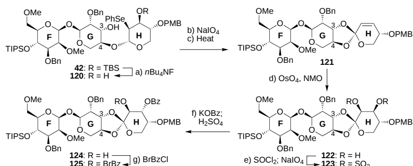
Scheme 14. Synthesis of FGH intermediates 124 and 125 . a) 1.05 equiv n Bu 4 NF, THF, 0 °C, 15 min, 82 % based on 85 % conversion; b) 10.0 equiv NaIO 4 , 8.0 equiv NaHCO 3 , MeOH/CH 2 Cl 2 /H 2 O 3:2:1, 25 °C, 4 h; c) vinyl acetate/toluene/diisopropylamine 2:2:1, sealed tube, 140 °C, 12 h, 74 % over two steps; d) 2.5 equiv NMO, 0.5 equiv OsO 4 , 1.0 equiv quinuclidine, Me 2 CO/H 2 O 10:1, 25 °C, 24 h, 65 %; e) 1.5 equiv SOCl 2 , 3.0 equiv Et 3 N, CH 2 Cl 2 , 0 °C, 5 min; 20 equiv NaIO 4 , 18 equiv NaHCO 3 , CCl 4 /MeCN/H 2 O 1:1:1.5, 0 → 25 °C, 1 h, 97 % over two steps; f) 3.0 equiv BzOK, 1.0 equiv [18]crown-6, DMF, 120 °C, 1 h; then 0.5 N H 2 SO 4 and 0.5 N H 2 O in THF, THF, 0 °C, 0.5 h, 76 %; g) 1.4 equiv BrBzCl, 4.0 equiv Et 3 N, 0.2 equiv 4-DMAP, CH 2 Cl 2 , 0 → 25 °C, 12 h, 100 %.
