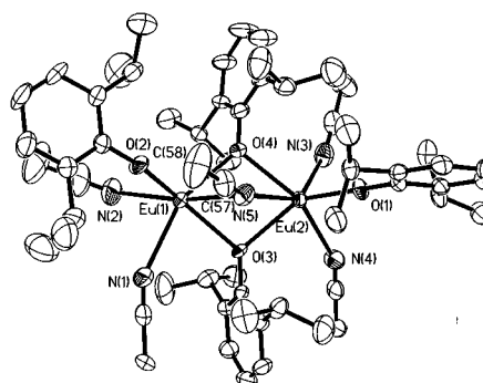
Fig. 2 Thermal ellipsoid plot of Eu 2 (OC 6 H 3 Pr 2 -2,6) 4 (NCCH 3 ) 5 2 with thermal ellipsoids drawn at the 50% probability level and hydrogen atoms omitted for clarity.
