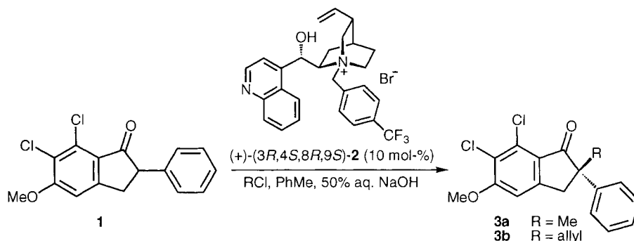
Scheme 1. Phase-Transfer-Catalyzed Alkylation of Phenylindanone 1 [10].
