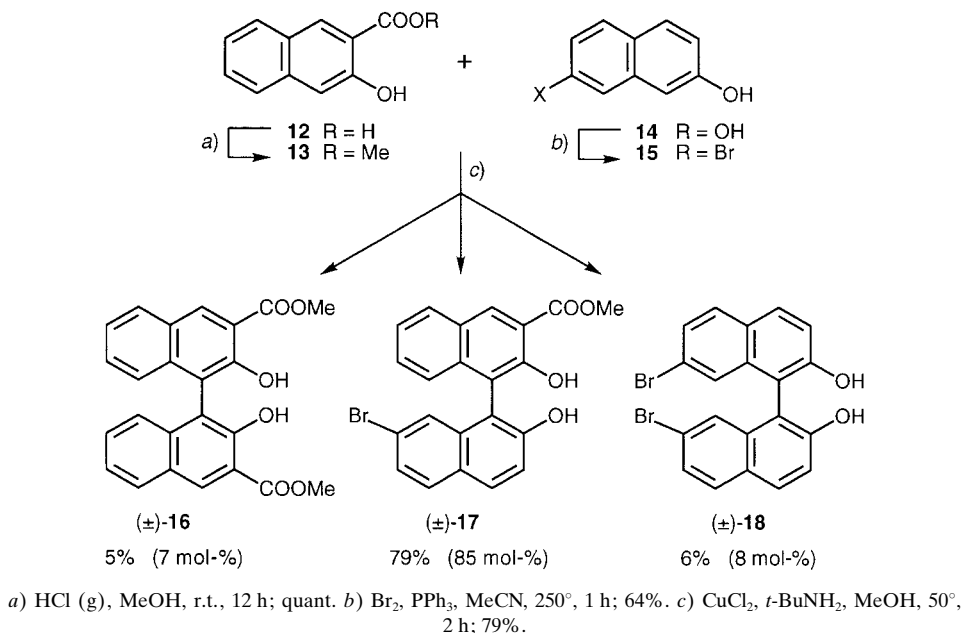
Scheme 3. Synthesis of 1,1'-Binaphthalene ( \pm )- 17 by \text{Cu}^{\text{II}} -Mediated Cross-Coupling
