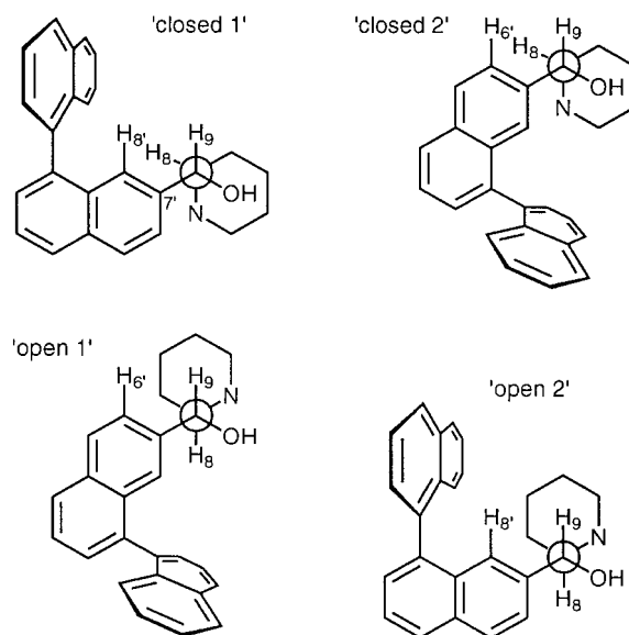
Fig. 3. Newman projections of the C(8)–C(9) bond for the four possible conformations of diastereoisomer (+)- 30 . The MeO and \text{MeOCH}_2 substituents on the 1,1'-binaphthalene were omitted for clarity. The three other diastereoisomers (+)- 29 , (–)- 31 , and (+)- 32 also adopt these four conformations; however, due to differences in the configuration at C(8) and C(9) , the orientation of \text{H}–C(9) with respect to \text{H}–C(8) and with respect to the naphthalene protons \text{H}–C(6') and \text{H}–C(8') may vary.
