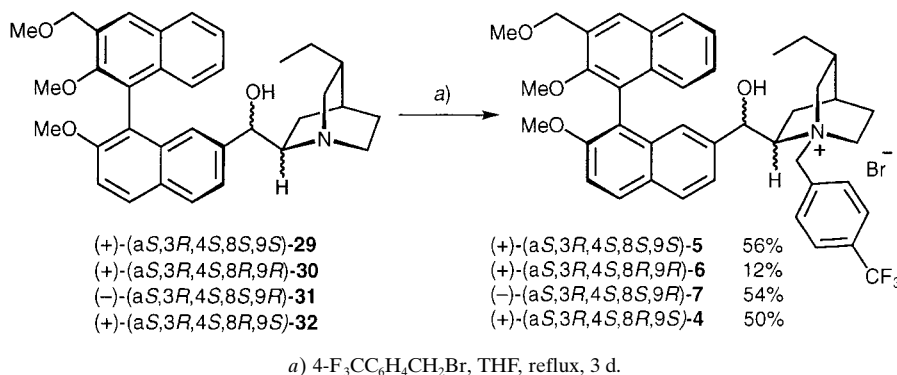
Scheme 7. Formation of the Novel Phase-Transfer Catalysts by Quaternization
