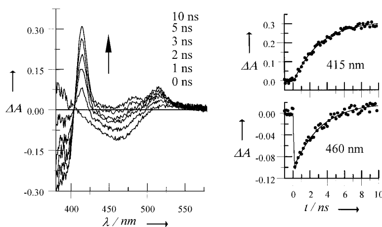
Figure 7. Transient differential absorption spectra recorded at various times after excitation of pyr–Pt–Ru in deoxygenated acetonitrile with a 25 ps laser pulse at 532 nm. Spectra were recorded at delay times of 0, 1, 2, 3, 5, and 10 ns. Also shown are kinetic traces obtained by overlaying spectral data collected at different delay times. Formation of triplet pyrene can be monitored at 415 nm while decay of the triplet state localized on the “Ru(bpy)” fragment can be followed at 460 nm. Solid lines drawn through the data points correspond to first-order kinetic processes with lifetimes of 2.9 and 3.1 ns, respectively, at 415 and 460 nm.
