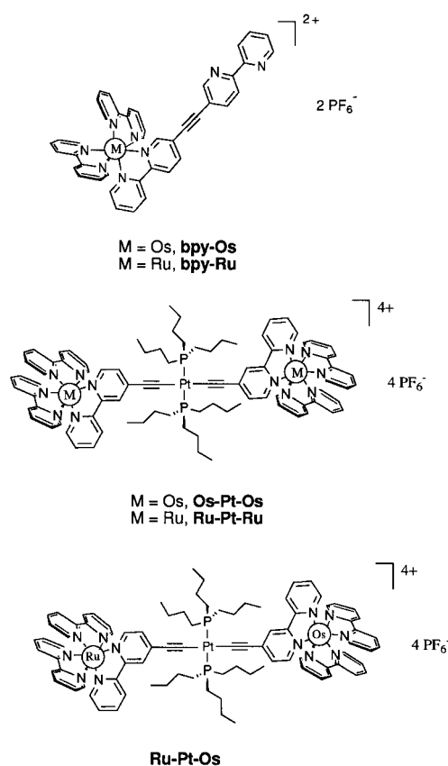
Scheme 5. Structures of the reference compounds.
