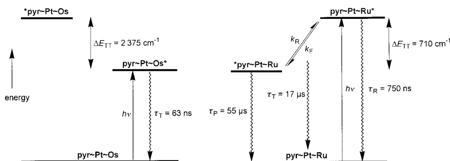
Figure 2. Simplified energy level diagrams for pyr–Pt–Os (left) and pyr–Pt–Ru (right). The triplet energy of the metal complex was established by fitting the emission spectrum recorded at 20 °C while the triplet energy for the pyrene unit was derived by kinetic spectrophotometry. Similar diagrams can be drawn for the corresponding pyr–Os and pyr–Ru systems.
