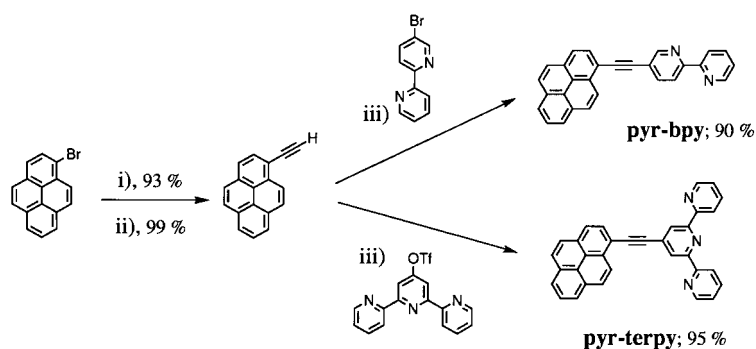
Scheme 1. i) Trimethylsilylacetylene, n -propylamine, [\text{Pd}(\text{PPh}_3)_4] (6 mol %), 60 °C, 24 h; ii) KF, CH 3 OH, 72 h; iii) benzene, diisopropylamine, [\text{Pd}(\text{PPh}_3)_4] (6 mol %), 80 °C, 24 h.
