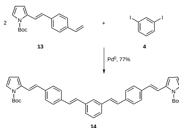
Scheme 4. Synthesis of 14 .
