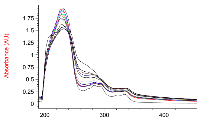
Figure 3. UV spectra of 1d (25.0 \mu\text{M} in 10 mM Tris-EDTA, pH=5.48) in the presence of varying concentrations of CT-DNA: 0, 0.25, 0.5, 1.0, 2.0, 4.0, 5.0, 10.0, 15.0, 20.0, 25.0, 30.0, 40.0, 50.0, 100 \mu\text{M} .
