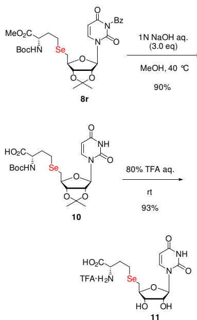
Scheme 3 Synthesis of Se-uridyl-L-selenohomocysteine ( 11 ).
