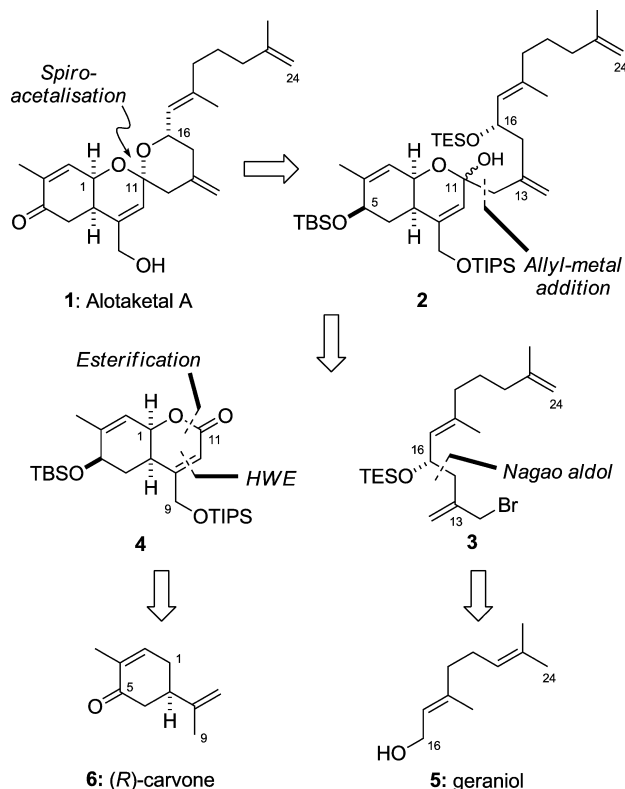
Scheme 1. Retrosynthetic Analysis of Alotaketel A
