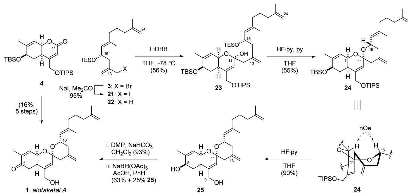
Scheme 5. Total Synthesis of Alotaketal A ( 1 )
