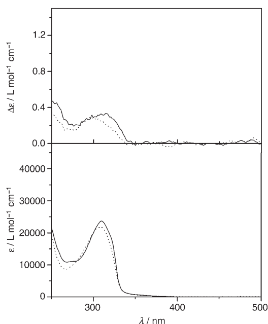
Figure 7. UV/Vis (bottom) and CD (top) spectra of solutions of the complexes 3 (---) and 4 (—) in \text{CH}_2\text{Cl}_2 .
