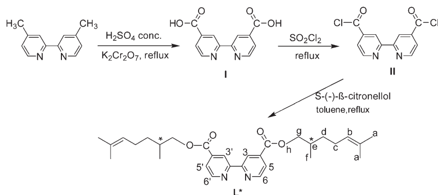
Scheme 1. Preparation of the \text{L}^* ligand.
