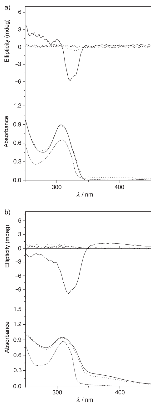
Figure 8. UV (lower) and CD (upper) spectra of 3 (a) and 4 (b) under different conditions: Diluted solution in \text{CH}_2\text{Cl}_2 (---), thin film in the mesophase at 25 °C (—), and in the isotropic phase at 100 °C (---).
