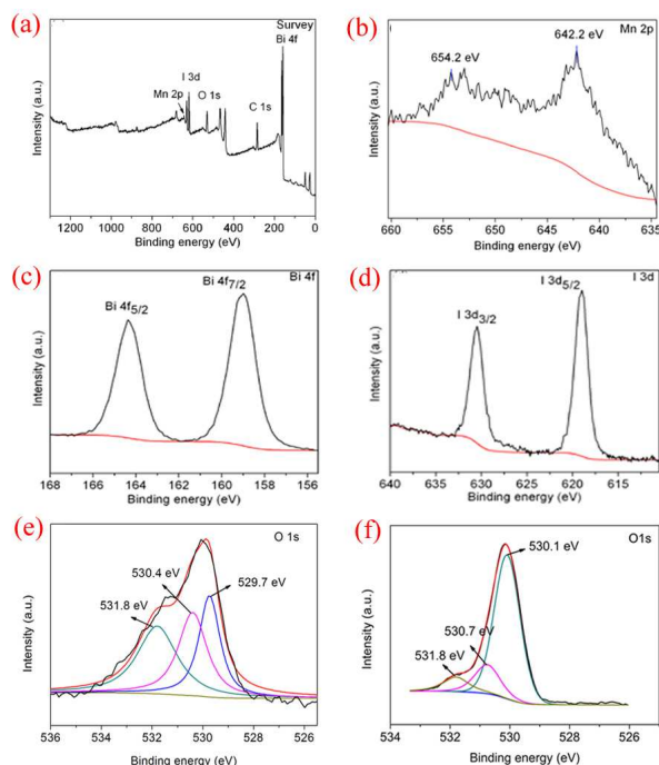
Fig. 2 The survey XPS of \text{MnO}_2/\text{BiOI} (4/5) (a), high resolution XPS of Mn 2p (b), Bi 4f (c), I 3d (d), O 1s (e) in \text{MnO}_2/\text{BiOI} (4/5), and O 1s (f) in \text{MnO}_2 + \text{BiOI} (4+5)
