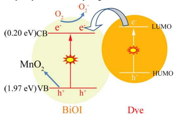
Fig. 9 The proposed possible mechanism for the improvement of photocatalytic activity
