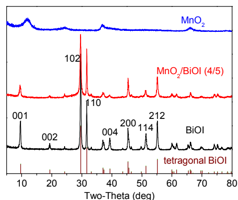
Fig. 1 XRD patterns of the as-prepared BiOI, \text{MnO}_2/\text{BiOI} (4/5), and \text{MnO}_2
