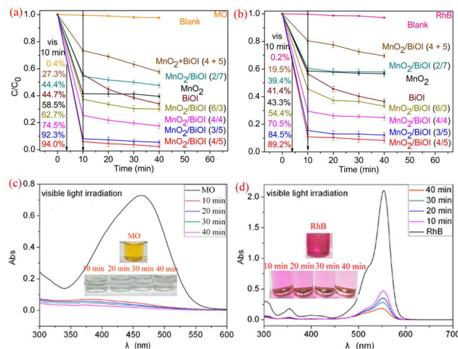
Fig. 6 Photodegradation of MO (a) and RhB (b) as a function of irradiation time; UV-Vis spectral changes of MO (c) and RhB (d) as a function of irradiation time over MnO 2 /BiOI (4/5)
