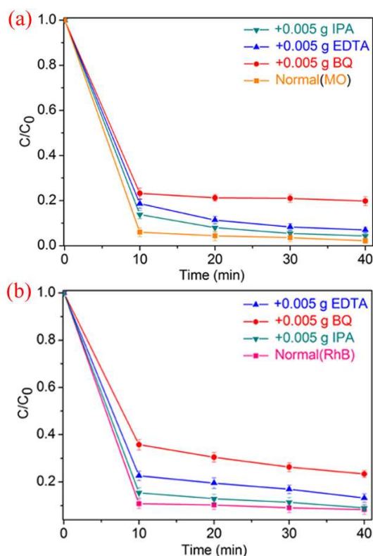
Fig. 8 Effects of different scavengers on the degradation of MO (a) and RhB (b) over MnO 2 /BiOI (4/5) composite
