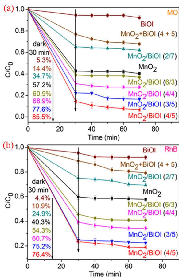
Fig. 5 Adsorption of MO (a) and RhB (b) as a function of time under dark condition
