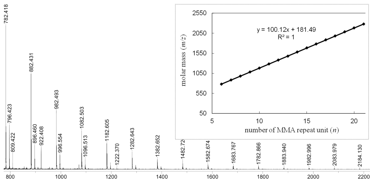
Figure 11. MALDI-TOF MS spectrum of low-molecular-weight MMA oligomers produced by I t Bu in DMF at RT. Inset: plot of m/z values of the major mass series vs the number of MMA repeat units ( n ).
