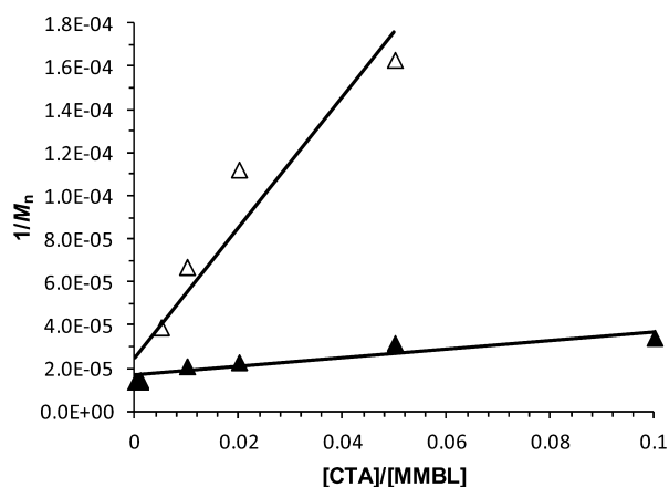
Figure 13. Plots of 1/M_n vs [CTA]/[M] ( M = \text{MMBL} ) for chain-transfer polymerization of MMBL by I t Bu. CTA = DMM (Δ); MBO (▲).
