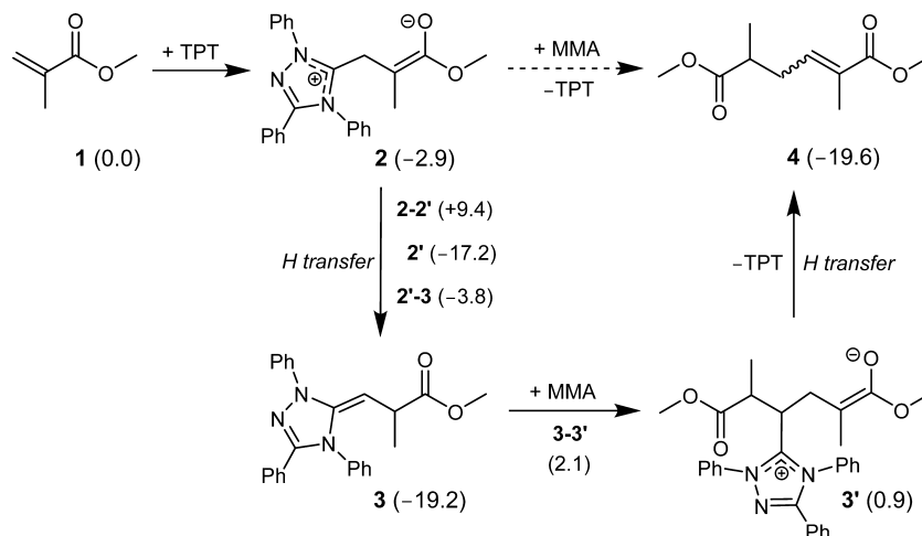
Scheme 6. Energetics for the Species Involved in the Termination Step of MMA Polymerization by i Bu in DMF a
