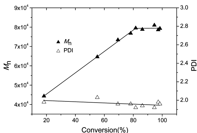
Figure 4. Plots of M_n and PDI of PMMBL vs MMBL conversion in DMF at 25 °C: [\text{MMBL}]_0 = 0.935\text{ M} , [\text{I}^t\text{Bu}] = 0.0936\text{ mM} with a [\text{MMBL}]_0/[\text{I}^t\text{Bu}]_0 ratio of 10 000/1.
