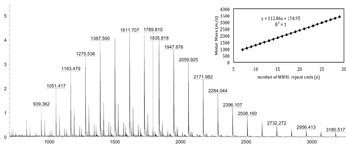
Figure 14. MALDI-TOF MS spectrum of low-molecular-weight MMBL oligomers produced by t^t\text{Bu} with DMM as the CTA. Inset: plot of m/z values of the major mass series vs the number of MMBL repeat units ( n ).
