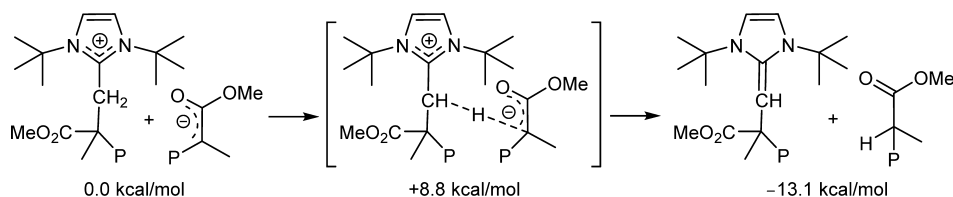
Scheme 6. Energetics for the Species Involved in the Termination Step of MMA Polymerization by i Bu in DMF a
