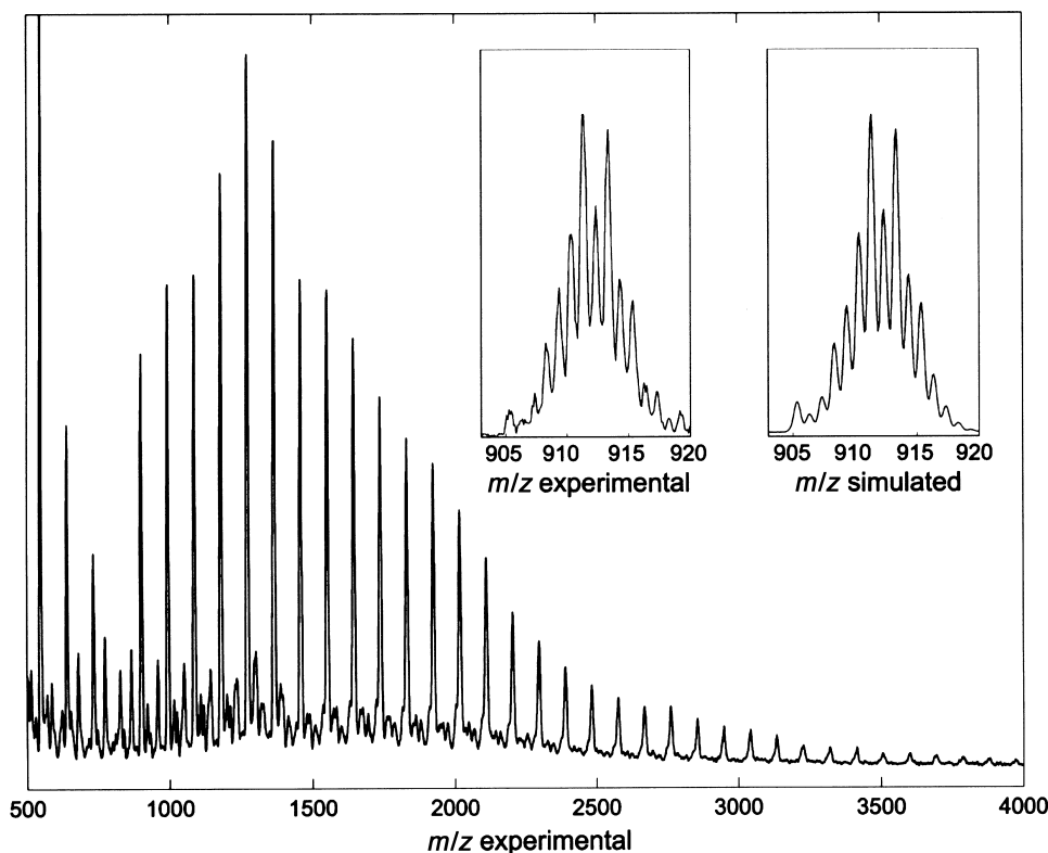
Fig. 1. ROMP of 5 equiv. of norbornene with 1 and 2a as fishhook. The polymer distribution with n = 0 starts at m/z 911. The ESI-MS was performed on a Finnigan MAT TSQ-700 by electrospraying at 10^{-5} M solution of the labelled living catalyst in \text{CH}_2\text{Cl}_2 in high-mass mode. Tube lens voltage was 170 V. The two insets show the experimental and computed isotope distributions for one of the oligomer peaks, which indicate, along with the mass, that the complex has one ruthenium, one phosphine, two chlorines, and one unit of the cation in 2a .
