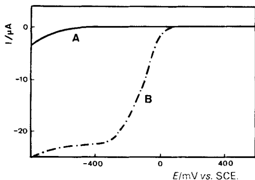
Fig. 7. Current-potential curves for the reduction of a saturated solution of oxygen at a clean (A), and a coated (B), rotating disc glassy carbon electrode (supporting electrolyte: 1M H_2SO_4 , rotation rate: 50 Hz)
