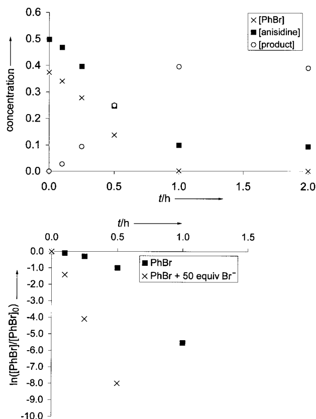
Figure 1. Plot of concentration versus time for the reaction of 2-methoxyaniline with bromobenzene catalyzed by complex 1e (top) and first-order plot of the decay of bromobenzene with Br^- (50 equiv) and without additional Bu_4NBr (bottom).
