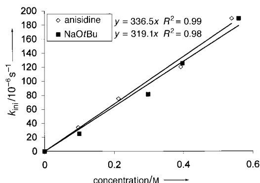
Figure 6. Plots of k_{\text{ini}} [a] versus [NaOtBu] and [o-anisidine] for the coupling of o -anisidine with phenyltrifluoromethane sulfonate in toluene at 298 K catalyzed by 2e . [b] [a] Measured after six minutes. [b] For experimental details: see Experimental Section.
