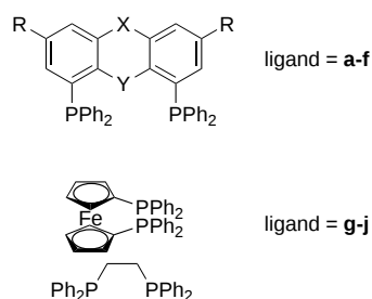
Scheme 2. Structures of phosphane ligands: a = DPEphos, X = H, H, Y = O, and R = H; b = Homoxantphos, X = \text{CH}_2\text{CH}_2 , Y = O, and R = H; c = Sixantphos, X = \text{Si}(\text{CH}_3)_2 , Y = O, and R = H; d = Thioxantphos, X = S, Y = O, and R = \text{CH}_3 ; e = Xantphos, X = \text{C}(\text{CH}_3)_2 , Y = O, and R = H; f = Thioxantphos, X = \text{C}(\text{CH}_3)_2 , Y = S, and R = H; g = dppf; h = dppe; i = \text{PPh}_3 ; j = \text{P}(o\text{-tolyl})_3 .
