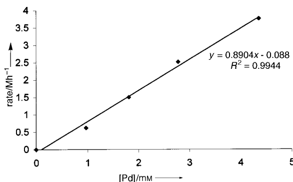
Figure 4. Plot of the rate [a] versus [Pd] for the reaction of 2-methoxyaniline with bromobenzene in toluene at 298 K catalyzed by 1e in presence of 50 equivalents of tetrabutylammonium bromide. [b] [a] rate = d[\text{product}]/dt , measured after six minutes. [b] For experimental details: see Experimental Section.
