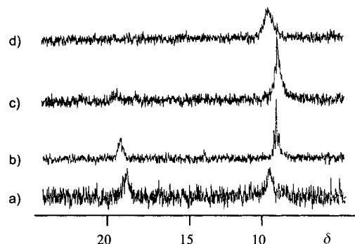
Figure 7. ^{31}\text{P}\{^1\text{H}\} NMR spectra of a mixture of complex 1e , bromobenzene, 2-methoxyaniline, and sodium tert -butoxide in [\text{D}_8]\text{toluene} recorded successively at a) 193 K, b) 273 K, c) 353 K, and d) 233 K.
