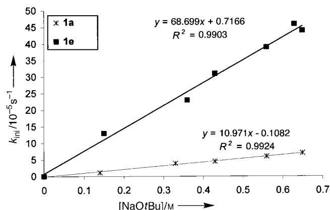
Figure 2. Plot of the k_{ini}^{[a]} versus [NaOtBu] for the reaction of 2-methoxyaniline with bromobenzene in toluene at 313 K catalyzed by complexes 1e and 1a . [b] [a] Measured after six minutes. [b] For experimental details: see Experimental Section.
