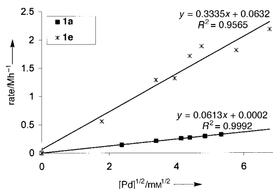
Figure 3. Plot of the rate [a] versus [Pd]^{1/2} with 1e and 1a for the reaction of 2-methoxyaniline with bromobenzene in toluene at 313 K. [b] [a] rate = d[\text{product}]/dt , measured after six minutes. [b] For experimental details: see Experimental Section.
