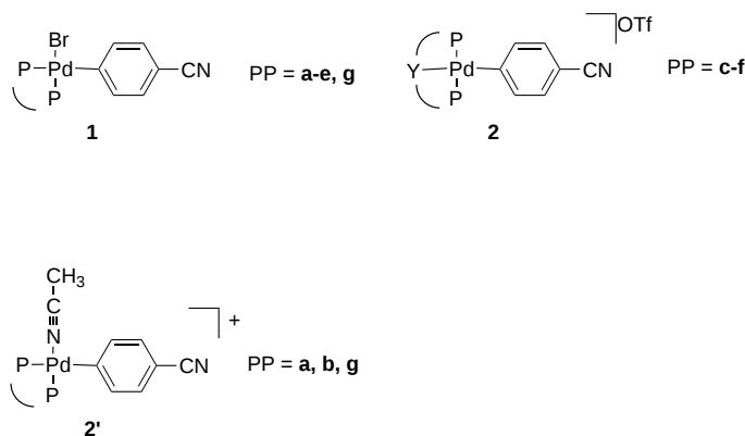
Scheme 3. [\text{Pd}^{\text{II}}(\text{PP})(p\text{-C}_6\text{H}_4\text{CN})] complexes (PP): 1a = DPEphos; 1b = Homoxantphos; 1c = Sixantphos; 1d = Thioxantphos; 1e = Xantphos; 1g = dppf; 2c = Sixantphos, and Y = O; 2d = Thioxantphos, and Y = O; 2e = Xantphos, and Y = O; 2f = Thioxantphos, and Y = S; 2'a = DPEphos; 2'b = Homoxantphos; 2'g = dppf.
