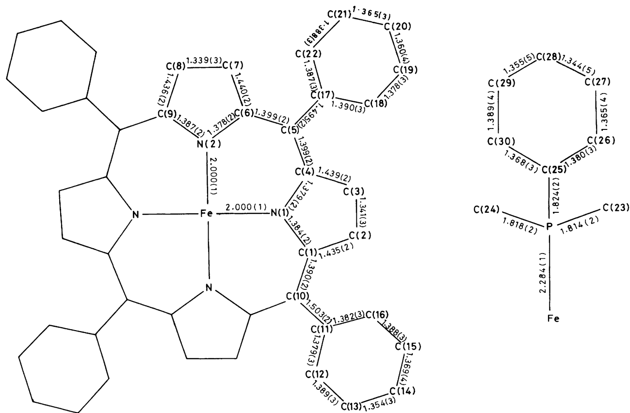
Figure 2. Atom labelling scheme for [\text{Fe}(\text{tpp})(\text{PMe}_2\text{Ph})_2] and the bond distances (Å) of the co-ordination group
