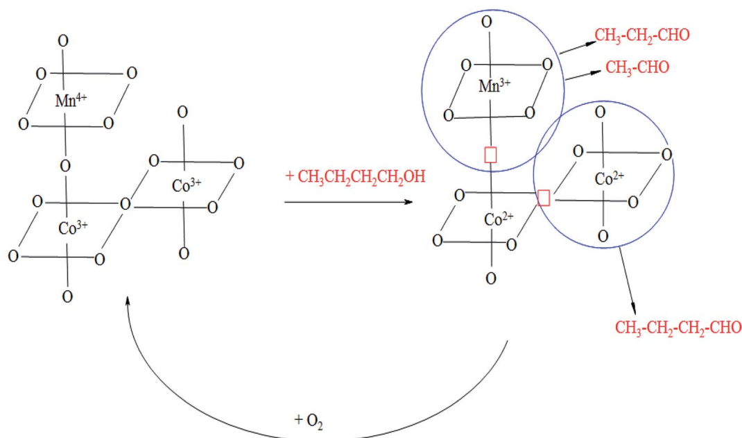
Scheme 1 Selective oxidation of n -butanol over \text{MnCo}_2\text{O}_4 spinel.
