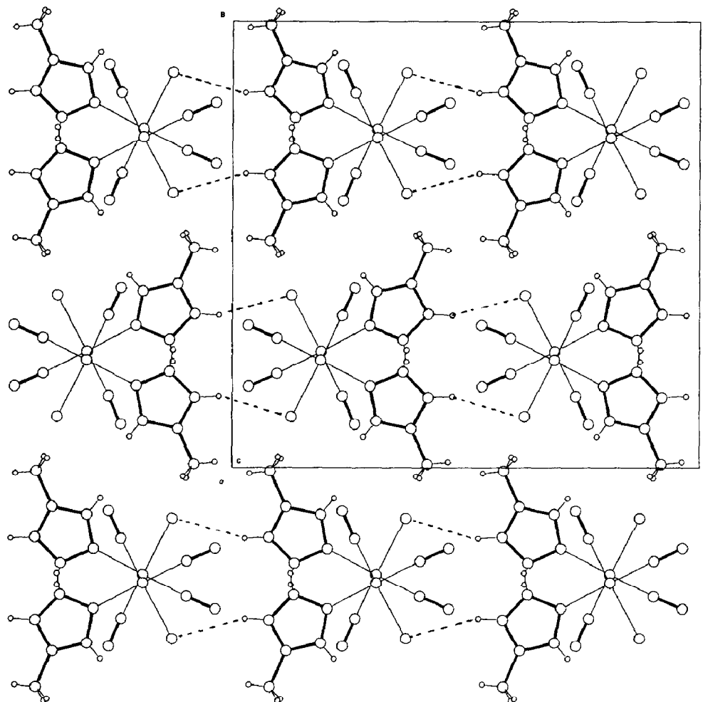
Fig. 2. Molecular packing of the title compound projected along the c -axis showing the Cl \cdots H-C contacts and the disposition of the planar coordinations.
