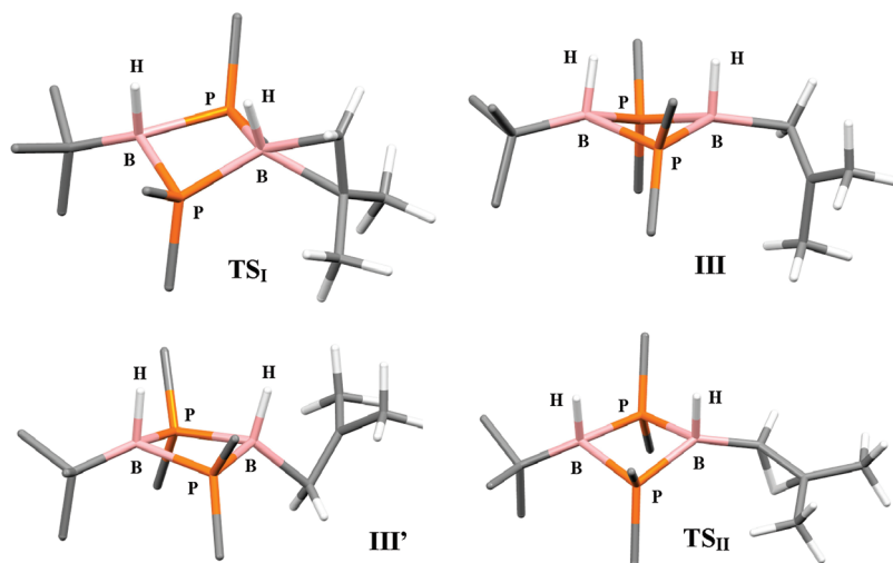
Figure 9. Optimized geometries for \text{TS}_\text{I} , III , III' , and \text{TS}_\text{II} .
