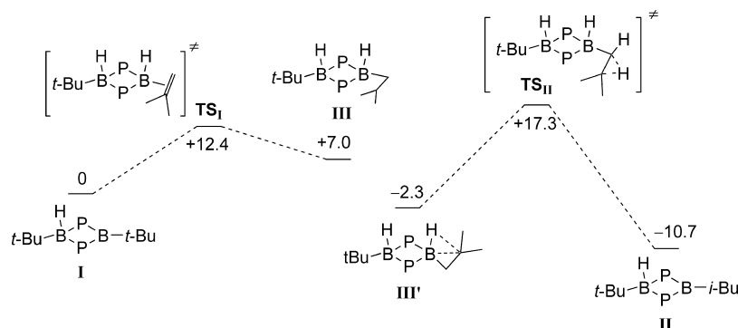
Figure 8. Energy profile computed at the B3PW91/SDD(P,Cl),6-31G** (B,C,H) level of theory (free energies G at 25 °C including ZPE correction in kcal/mol) for the t\text{-Bu} \rightarrow i\text{-Bu} isomerization from I to II ( i\text{-Pr} substituents at phosphorus and atomic charges omitted for clarity).
