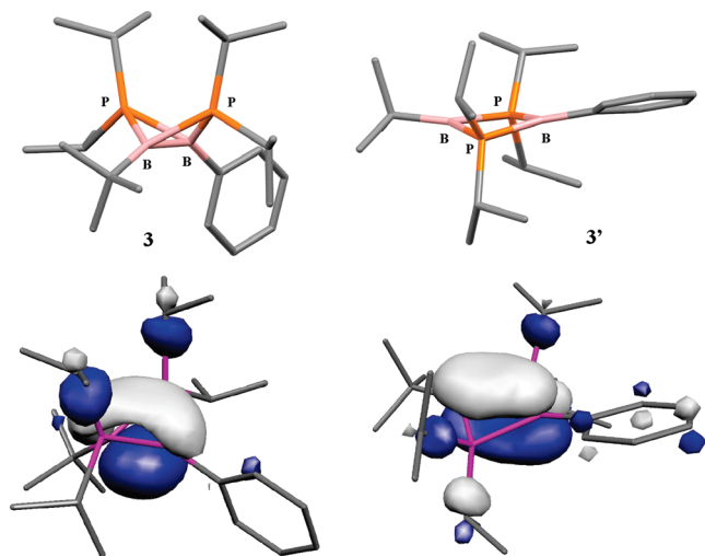
Figure 3. Optimized geometries and Kohn–Sham representations of the HOMO orbitals for the 1,3-dibora-2,4-diphosphoniobicyclo[1.1.0]butane 3 and the corresponding 1,3-dibora-2,4-diphosphoniocyclobutane-1,3-diyl structure 3' .
