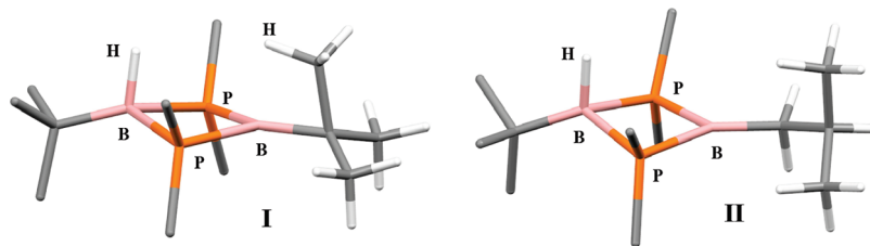
Figure 7. Optimized geometries for I and II .
