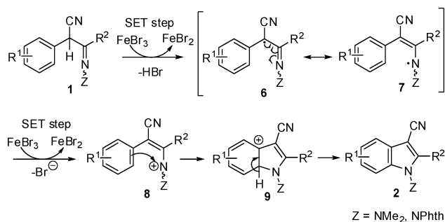
Scheme 2 Proposed mechanistic pathway.
