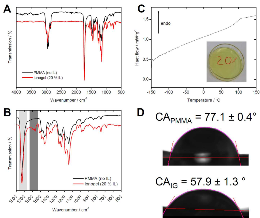
Figure 2. (A) Full IR spectrum of the PMMA matrix and an ionogel with 20% of IL. (B) Magnified view of the low wavenumber region. (C) DSC curve of the ionogel.. Inset is a photograph of the ionogel. (D) Photographs of a water droplet on the pure PMMA ( CA_{PMMA} ) and the ionogel ( CA_{IG} ) showing the different contact angles.
