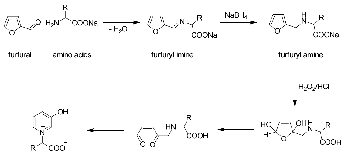
Fig. 2 Synthetic route for the pyridinium zwitterions from furfural and amino acids.
