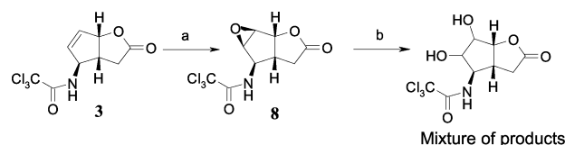
Scheme 4 Epoxidation of 3 . Reagents and conditions: a) m -CPBA, \text{CH}_2\text{Cl}_2 , reflux, 4 d (98%); b) aq. HCl (4 M), 90^\circ\text{C} , 4 h.
