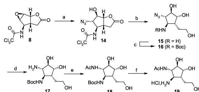
Scheme 9 Synthesis of the potential \beta -D- N -acetylglucosaminidase inhibitor 19 . Reagents and conditions: a) \text{NaN}_3 , \text{NH}_4\text{Cl} , DMF, 80^\circ\text{C} , 1.5 h (65%); b) \text{CaCl}_2 , \text{NaBH}_4 , THF, -20^\circ\text{C} , overnight; c) \text{Boc}_2\text{O} , \text{NaHCO}_3 , acetone, \text{H}_2\text{O} , rt, overnight (40%); d) \text{H}_2 , 5% \text{Pd/C} , ethanol, rt, 2.5 h; e) \text{H}_2\text{O} -MeOH (1 : 2), \text{Ac}_2\text{O} , rt, 1 h (80%); f) aq. \text{HCl} (4 M), rt, 15 min (quant.).
