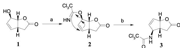
Scheme 2 Overman rearrangement. Reagents and conditions: a) \text{Cl}_3\text{CCN} , NaH, THF, 0^\circ\text{C} , 1 h; b) xylene, reflux, 2 h (75%, 2 steps).
