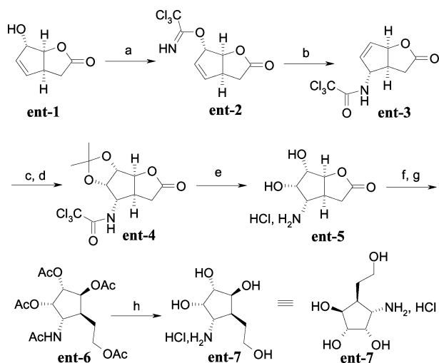
Scheme 6 Synthesis of aminocyclopentanol ent-7 . Reagents and conditions: a) \text{Cl}_3\text{CCN} , \text{NaH} , THF, 0^\circ\text{C} , 2 h; b) xylene, reflux, 3 h (43%, 2 steps); c) \text{OsO}_4 , NMO, \text{CH}_2\text{Cl}_2 , rt, overnight; d) 2,2-dimethoxypropane, acetone, conc. \text{H}_2\text{SO}_4 , rt, 2 h (72%); e) aq. \text{HCl} (6 M), reflux, 2.5 h (79%); f) \text{Ca}(\text{BH}_4)_2 , ethanol, -20^\circ\text{C} , overnight; g) \text{Ac}_2\text{O} , pyridine, rt, overnight (42%); h) aq. \text{HCl} (4 M), 60^\circ\text{C} , 4.5 h (quant.).
