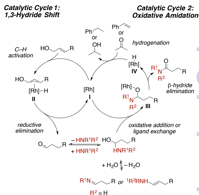
Scheme 4. Proposed dual catalytic cycle.
