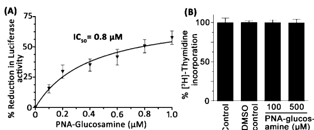
Figure 5. (A) Inhibition of HIV-1 transcription by 5a : The CEM cells were infected with pseudotyped HIV-1 virus expressing the firefly luciferase reporter. After 48 h postinfection, indicated amount of PNA–aminoglucosamine was supplemented in the culture medium. After 76 h, cells were harvested and assayed for firefly luciferase activity in the cell extract. The results are expressed as mean value of two independent experiments with error bar. (B) Effect of 5a on cellular proliferation: CEM cells were grown in the absence or presence of 0.1 mM and 0.5 mM of 5a dissolved in DMSO. The final concentration of DMSO supplemented through 5a in the medium was 5%. The culture medium was supplemented with 5 \mu Ci of [methyl- 3 H]thymidine/mL. After 48 h, cells were harvested and [ 3 H]-thymidine incorporated into the DNA was determined. The results expressed as percent of thymidine incorporation with respect to the control are the averages of three sets of independent experiments.
