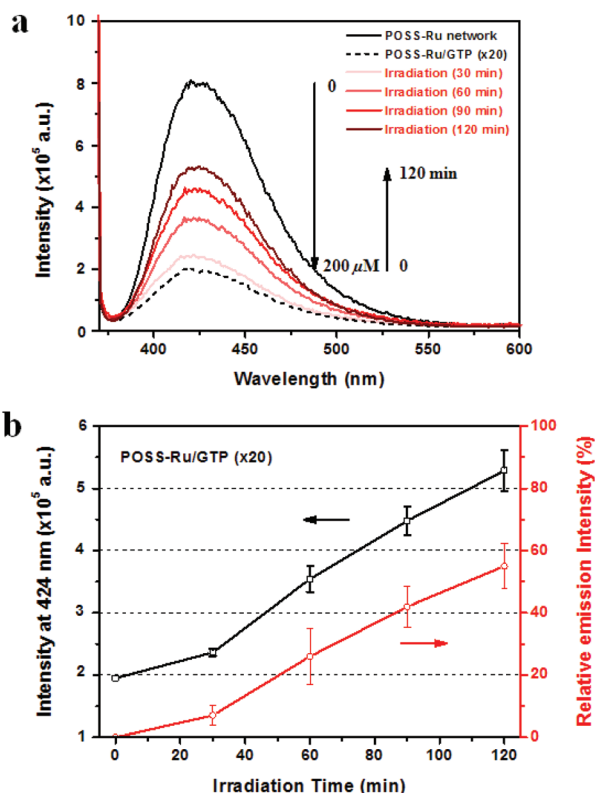
Fig. 5 (a) Emission changes of 10 \mu\text{M} naphthyridine ligands in POSS-Ru by adding 200 \mu\text{M} GTP with 100 \mu\text{M} \text{K}_3[\text{Fe}(\text{CN})_6] in PBS buffer solution (pH 7.4) at 25 ^\circ\text{C} . Excitation wavelength was 364 nm. Photoreaction was performed for 120 min at 25 ^\circ\text{C} with a 4 W UV-lamp (365 nm). (b) The profile was obtained in PBS buffer solution for GTP in the POSS-Ru/GTP complex under UV irradiation.
