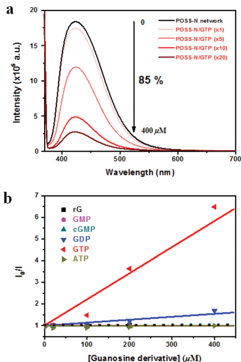
Fig. 2 (a) Emission changes of 20 \mu\text{M} naphthyrindine ligands in POSS-N by adding GTP (0 to 400 \mu\text{M} ) in PBS buffer solution (pH 7.4) at 25 ^{\circ}\text{C} . Excitation wavelength was 364 nm. (b) Stern–Volmer plots with the solution containing 20 \mu\text{M} naphthyrindine ligand in POSS-N by adding various kinds of guanosine nucleosides.
