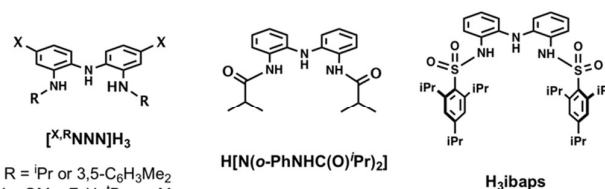
Figure 1. Comparison of the H 3 ibaps ligand used in this work with other reported redox non-innocent [NNN]-pincer ligands.
