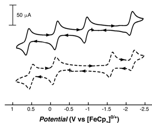
Figure 2. Cyclic voltammograms of 1 (solid) and [Ga III (ibaps)bpy] (dashed) at room temperature in CH 3 CN.
