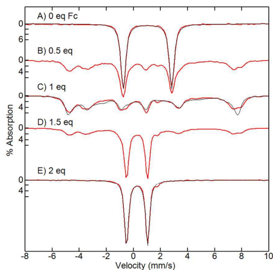
Figure 5. Mössbauer spectra (red traces) and simulations (black traces) of a titration of 1 (A) with ferrocenium (equivalents as shown), recorded at 4.2 K in a magnetic field of 50 mT. For C, the simulation is for an S = 2 \text{Fe}^{\text{II}} exchanged coupled to S = \frac{1}{2} with \text{Fe}^{\text{II}} parameters of D = 3.5 \text{ cm}^{-1} , E/D = 0.16 , A = (-21, -30, -36) \text{ MHz} , \delta = 0.69 \text{ mm/s} , \Delta E_{\text{Q}} = 2.55 \text{ mm/s} .
