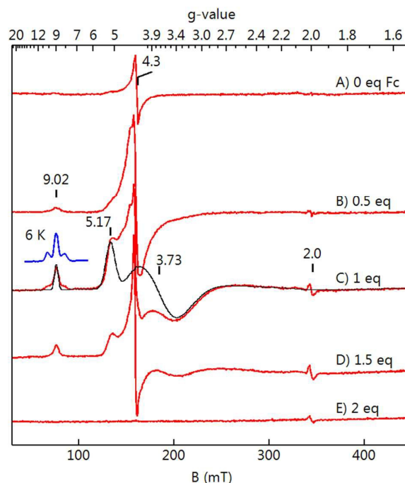
Figure 6. EPR spectra (red traces, 9.646 GHz, 0.2 mW) and simulations (black trace) of a titration of 1 (A) with ferrocenium (equivalents as shown) recorded at 16 K. The simulation is for an S = 2 \text{Fe}^{\text{II}} exchanged coupled to S = \frac{1}{2} with \text{Fe}^{\text{II}} parameters of D = 3 \text{ cm}^{-1} , E/D = 0.19 .
