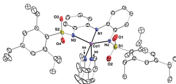
Figure 3. Thermal ellipsoid diagram of 1-Co . The ellipsoids are drawn at the 50% probability level, and hydrogen atoms are omitted for clarity.
