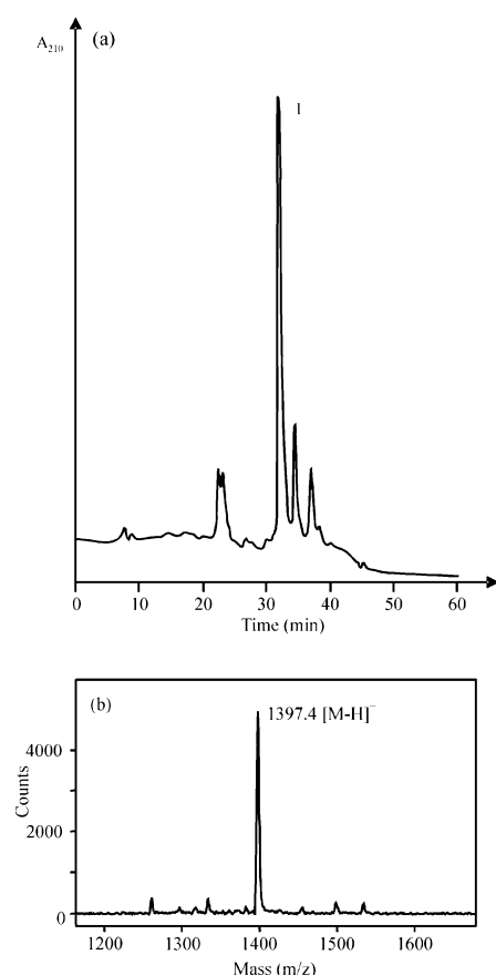
Fig. 3 Crude MAP Kinase ERK2 [178–188; Thr( P ) 183 , Tyr( P ) 185 ] ( 13 ), (a) RP-HPLC, (b) MALDI-MS (peak 1).
