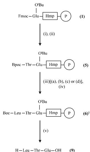
Scheme 3 Reagents and conditions: (i) 25% piperidine–DMF (20 min), (ii) Bpoc–Thr–OH (3 eq.)–HBTU (3 eq.)–NMM (9 eq.) (1 h), (iii) formic acid–DCM [(a) 5%, (b) 10%, (c) 15% or (d) 20%; 20 min], (iv) Boc–Leu–OH (3 eq.)–HBTU (3 eq.)–NMM (9 eq.) (1 h), (v) TFA–TES–H 2 O (95 : 2.5 : 2.5, v/v/v; 1 h).
