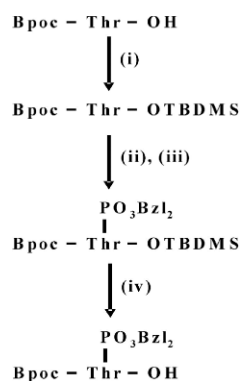
Scheme 1 Reagents and conditions: (i) TBDMSCl (0.9 eq.)–NMM (1 eq.) in THF (3 min), (ii) (BzlO) 2 PN i Pr 2 (1.2 eq.)–1 H -tetrazole (3 eq.) (2 h), (iii) 14% t BuOOH (30 min), (iv) 10% Na 2 S 2 O 5 (30 min).
