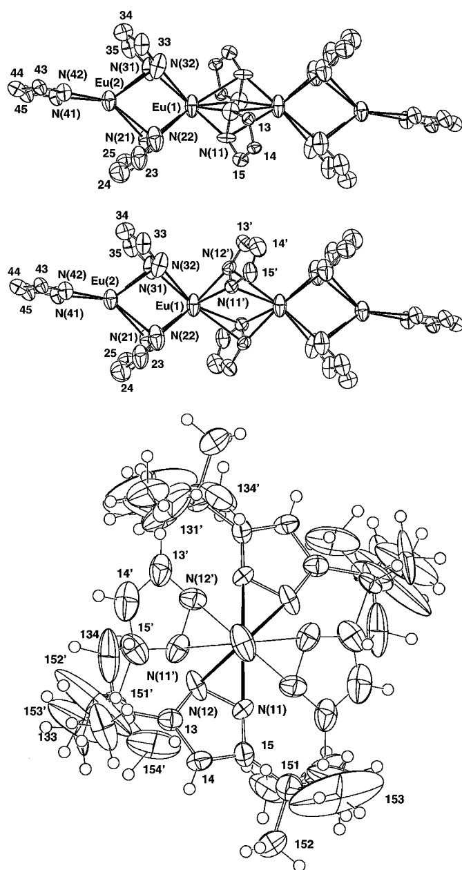
Figure 3. Top and middle: [Eu 4 (tBu 2 pz) 8 ] ( 6 ); the two deconvoluted components devoid of their tBu substituents. Bottom: The ligand environment between Eu(1) and Eu(1*) viewed down the Eu(1)⋯Eu(1*) line, both disordered components of ligand 1 and 1* being shown.
