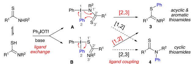
Scheme 4 Proposed mechanism for S - and N -arylation.
