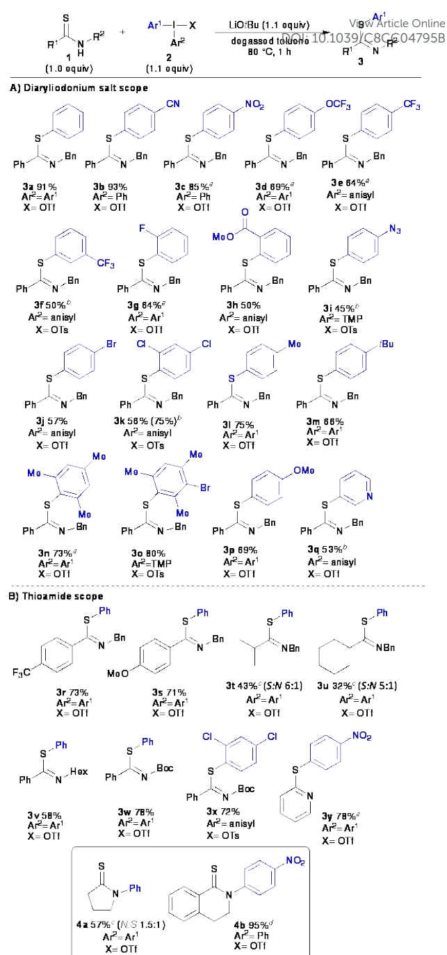
Scheme 2 Arylation scope with major isomer ( Z ) shown. Z:E ratios 91:9 to 96:4, except 3d (89:11), 3f (88:12), 3h (86:14), 3i (90:10), 3o (86:14), and 3q (87:13). Only one isomer obtained of 3v-4b . a In non-degassed toluene. b NMR yield. c Combined yield. d At rt for 16 h, 1.5 equiv base.
