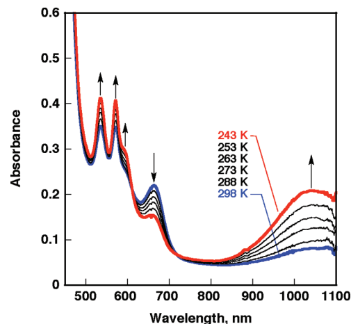
Figure 6. vis-NIR spectral changes of a \text{CH}_2\text{Cl}_2 solution of TPZn 3 ( 1.4 \times 10^{-5} M) in the presence of 2 equiv of [\text{Ru}(\text{bpy})_3]^{3+} at different temperatures.
