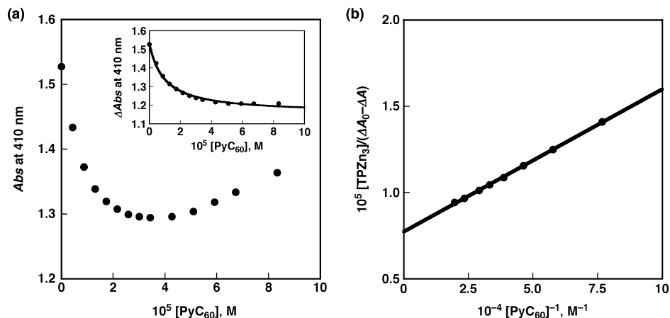
Figure 9. (a) Original spectral change at 410 nm due to TPZN 3 with increasing concentration of PyC 60 in o -dichlorobenzene at 298 K. Inset: \Delta\text{Abs} at 410 nm. (b) Plot of [\text{TPZN}_3]/(A_0 - A) vs [\text{PyC}_{60}]^{-1} .
