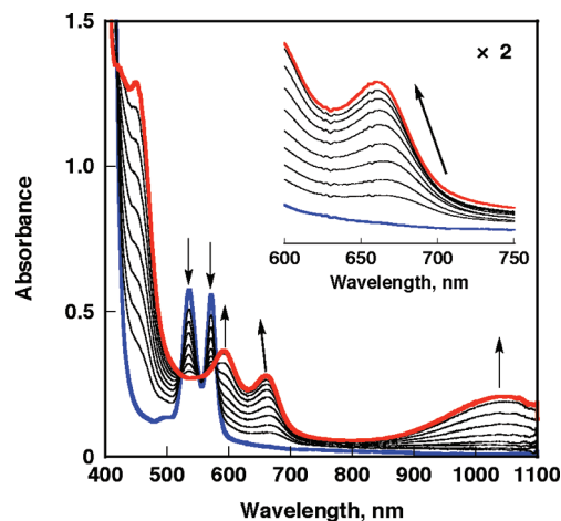
Figure 4. vis-NIR spectral changes upon addition of [\text{Ru}(\text{bpy})_3]^{3+} (up to 3 equiv) to a \text{CH}_2\text{Cl}_2 solution of TPZn 3 ( 1.7 \times 10^{-5} M) at 298 K.
