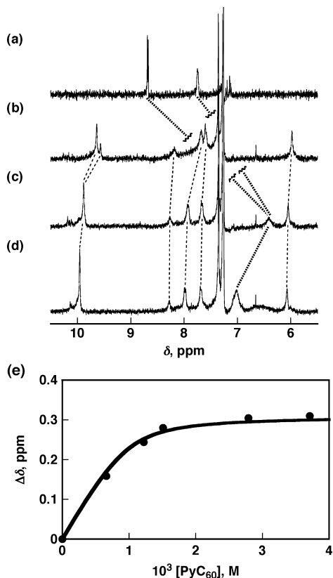
Figure 10. ^1\text{H} NMR spectra of (a) PyC 60 , (b) TPZN 3 ( 1.0 \times 10^{-3} M), and (c and d) TPZN 3 ( 1.0 \times 10^{-3} M) in the presence of PyC 60 ; (c) 1.2 \times 10^{-3} M and (d) 3.7 \times 10^{-3} M in \text{CDCl}_3/\text{CS}_2 (1:1 v/v ). The dashed lines represent the spectral changes due to TPZN 3 , whereas the dotted lines represent the spectral changes due to pyridine moieties of PyC 60 . (e) Change in the chemical shift of the meso -protons of TPZN 3 upon addition of PyC 60 . The curve represents the best fit according to eq 1.
