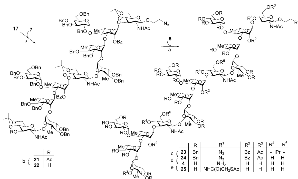
Scheme 4. Synthesis of the pentadecasaccharide hapten 25 bearing a masked-thiol-type of spacer. a) TfOH (cat.), MS, 1,2-DCE, -30^{\circ}\text{C} \rightarrow 5^{\circ}\text{C} , 2.5 h; b) MeONa (cat.), MeOH, room temperature, 3 h; c) 50% aqueous TFA, \text{CH}_2\text{Cl}_2 , 0^{\circ}\text{C} , 3 h; d) 1. MeONa (cat.), MeOH, 55^{\circ}\text{C} , overnight; 2. 10% Pd/C, 1 N aqueous HCl, EtOH/EtOAc, room temperature, 48 h; e) SAMA-Pfp, 0.1 M phosphate buffer (pH 7.4), room temperature, 2 h.
