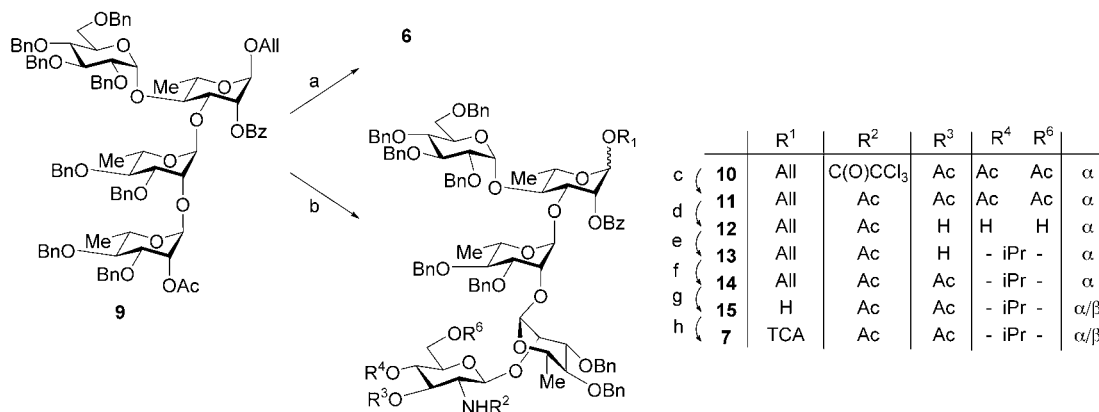
Scheme 2. Synthesis of building blocks 6 and 7 . a) 1. [Ir(cod){PCH 3 (C 6 H 5 ) 2 ] + PF 6 - (cat.), THF, room temperature, 2 h; 2. I 2 , THF/water, room temperature, 1 h; 3. CCl 3 CN, DBU, CH 2 Cl 2 , 0 °C, 1 h; b) see ref. [21]; c) Bu 3 SnH, AIBN (cat.), toluene, 100 °C, 1 h; d) MeONa (cat.), MeOH, room temperature, 25 min; e) Me 2 C(OMe) 2 , PTSA (cat.), DMF, room temperature, overnight; f) Ac 2 O, pyridine, room temperature, 2.5 h; g) 1. [Ir(cod){PCH 3 (C 6 H 5 ) 2 ] + PF 6 - (cat.), THF, room temperature, 2 h; 2. HgO, HgBr 2 , acetone/water, room temperature, 1 h; h) CCl 3 CN, DBU, CH 2 Cl 2 , 0 °C, 1 h. AIBN = 2,2'-azobisisobutyronitrile, All = allyl, cod = cycloocta-1,5-diene, DBU = 1,8-diazabicyclo [5.4.0]undec-7-ene, DMF = N,N -dimethylformamide, PTSA = p -toluenesulfonic acid, THF = tetrahydrofuran.
