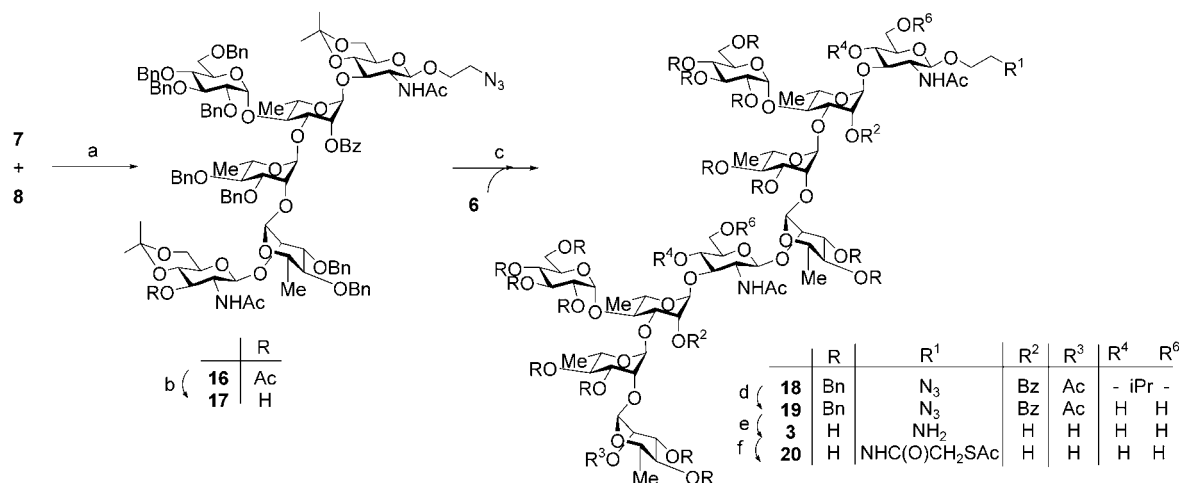
Scheme 3. Synthesis of the deca-saccharide hapten 20 bearing a masked-thiol-type spacer. a) TfOH (cat.), MS, 1,2-DCE, 75 °C, 2.5 h; b) MeONa (cat.), MeOH, room temperature, 3 h; c) TfOH (cat.), MS, 1,2-DCE, −35 °C→10 °C, 2.5 h; d) 50 % aqueous TFA, CH 2 Cl 2 , 0 °C; 3 h; e) 1. MeONa (cat.), MeOH, 55 °C, overnight; 2. 10 % Pd/C, 1 N aqueous HCl, EtOH/EtOAc, room temperature, 72 h; f) SAMA-Pfp, 0.1 M phosphate buffer (pH 7.4), room temperature, 1 h. 1,2-DCE = 1,2-dichloroethane, MS = 4 Å molecular sieves, SAMA-Pfp = S -acetylthioglycolic acid pentafluorophenyl ester, Tf = triflate = trifluoromethanesulfonyl, TFA = trifluoroacetic acid.
