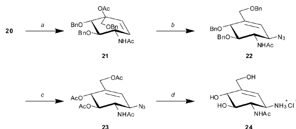
Scheme 4 (a) i. \text{PPh}_3 , \text{THF} , \text{H}_2\text{O} , ii. \text{Ac}_2\text{O} , \text{DMAP} , pyridine; (b) \text{Pd}(\text{PPh}_3)_4 , \text{NaN}_3 , \text{THF} , \text{H}_2\text{O} ; (c) i. \text{FeCl}_3 , \text{CH}_2\text{Cl}_2 , ii. \text{Ac}_2\text{O} , \text{DMAP} , pyridine; (d) i. \text{PPh}_3 , \text{THF} , \text{H}_2\text{O} , ii. \text{Boc}_2\text{O} , \text{KOH} , \text{MeOH} , iii. 6 M \text{HCl} , \text{MeOH} .
