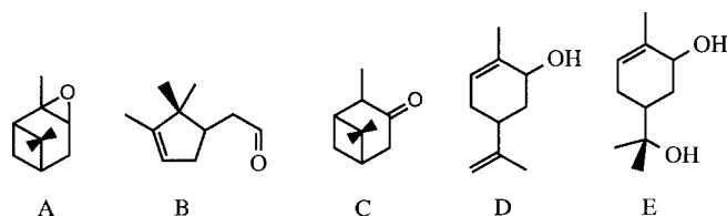
Figure 7. \alpha -Pinene oxide (A) and its decomposition products campholenic aldehyde (B), pinocampnone (C), trans -carveol (D), and trans -sobreolol (E).
