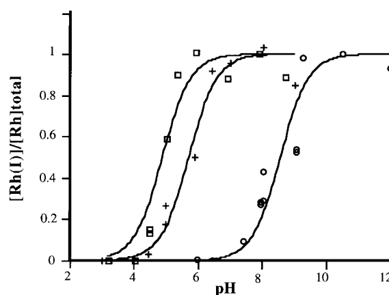
Figure 3. Fraction of the \text{Rh}^{\text{I}} complex as a function of pH for Rh-5 anchored to DODAC ( \square ), DPPC ( + ), and DHP ( \circ ) vesicles. Conditions: [surfactant] = 926 \mu\text{M} , [ Rh-5 ] = 72 \mu\text{M} .
