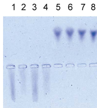
Fig. 5 Agarose gel shift assay: lanes 1 and 3 lysozyme, lanes 2 and 4 lysozyme and 1a , lanes 5 and 7 α-lactalbumin, lanes 6 and 8 α-lactalbumin and 1a .
