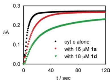
Fig. 6 Reduction kinetics of 10 μM cytochrome c by 2 mM ascorbate (5 mM phosphate, pH 7.4) in the presence and absence of receptors 1a and 1d .
