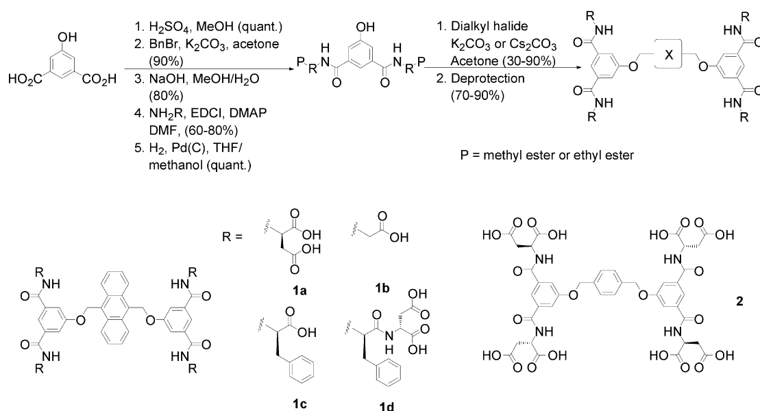
Scheme 1 Synthesis of receptors 1–2.
