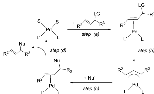
Scheme 1. Mechanism for the Palladium-Catalyzed Allylic Substitutions Using Soft Nucleophiles {S = Solvent, L and L' = Monodentate Ligands or (L,L') = Bidentate Ligand, LG = Leaving Group, Nu − = Nucleophile}
