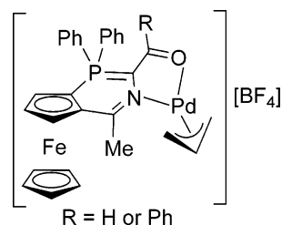
Figure 1. Palladium(II)-allyl complexes containing (N,O) ferrocenyl ligands used as precursors in allylic alkylation processes. 17
