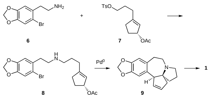
Scheme 1. Synthesis of cephalotaxine ( 1 ).
