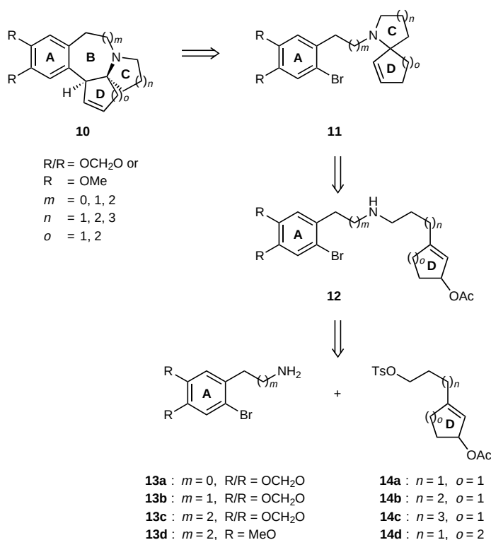
Scheme 2. Retrosynthesis of ring-size analogues 10 of cephalotaxine ( 1 ).
