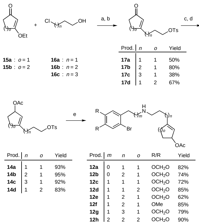
Scheme 3. Synthesis of the secondary amines 12 . a) MeMgCl (3.6 M in THF), THF, -78^{\circ}\text{C} → room temperature; then Mg, reflux; then 15a/b , -10^{\circ}\text{C} → RT; then NH 4 Cl solution; HCl (2 M); b) TsCl, py, -10^{\circ}\text{C} or TsCl, DMAP, Et 3 N, -10^{\circ}\text{C} ; c) DIBAL (1.5 M in toluene), toluene, -50^{\circ}\text{C} ; d) Ac 2 O, Et 3 N, DMAP, CH 2 Cl 2 , 0^{\circ}\text{C} ; e) 13 , TBAI (1.5 equiv), THF, reflux.
