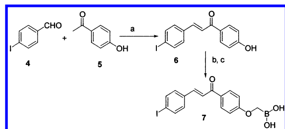
Scheme 2 b
