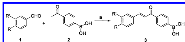
Scheme 1 a
