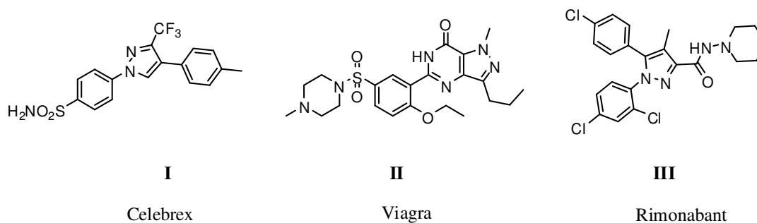
Figure 1. Some drugs incorporating pyrazole ring
