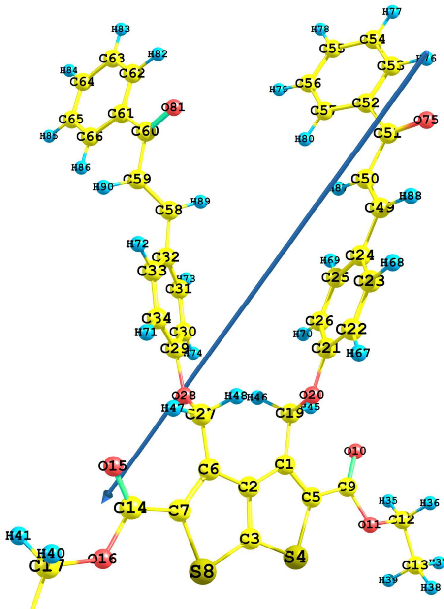
Figure 5. The optimized geometry, numbering system, the vector of the dipole moment and the moiety of addition of 10 using B3LYP/6-31G.
