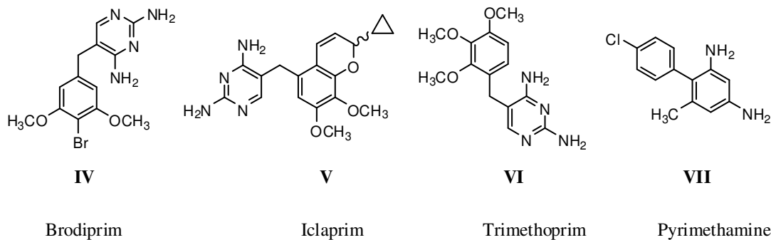
Figure 2. Some pyrimidine derivatives as antibacterial drugs
