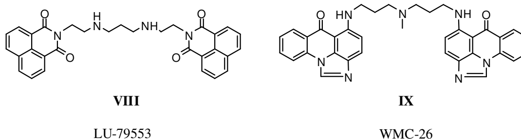
Figure 3. Some bis-heterocycles with anti-tumor activity
