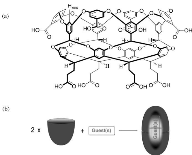
Fig. 1 a) Deep-cavity cavitand 1 . b) Schematic of the templated dimerization of 1 .
