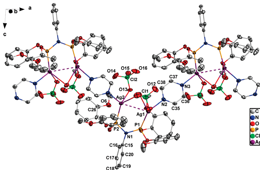
Figure 7. Molecular structure of 14 . All hydrogen atoms have been omitted for clarity. Displacement ellipsoids are drawn at the 50% probability level. View axes: -86.99^\circ , -22.32^\circ , -3.48^\circ . Symmetry operation i = -0.5 + x, y, 0.5 - z , ii = 0.5 + x, y, 0.5 - z .
