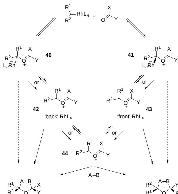
Scheme 9. Mechanistic analysis.
