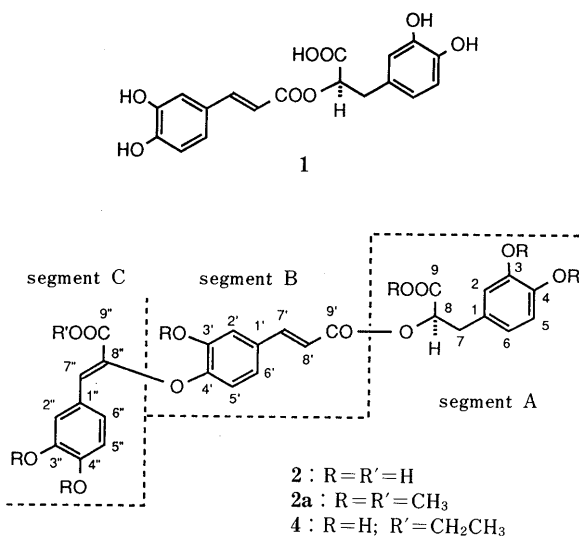
Chart 1. Structures of Rosmarinic Acid (1), Melitric Acid A (2), Dimethyl Penta-O-methylmelitrate (2a) and Ethyl Melitrate A (4)
