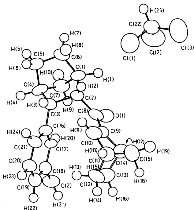
Fig. 1. X-Ray crystal structure of Ia·CHCl 3 ; perspective view of the molecule.
