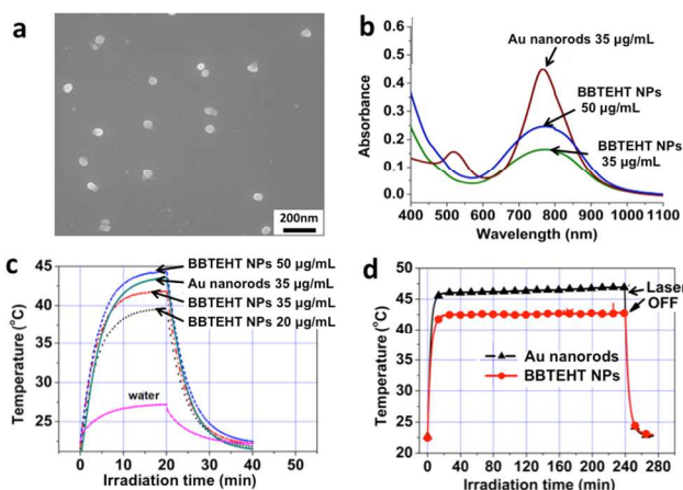
Fig. 1 a) SEM image of BBTEHT NPs from a dispersion of 35 µg/mL. b) UV-Vis-NIR spectra of BBTEHT NPs (35 and 50 µg/mL, respectively) and Au nanorods (35 µg/mL). c) Temperature change plots of different concentration BBTEHT NPs and Au nanorods under irradiation by an 808-nm laser with a power density of 1.77 \text{ W/cm}^2 for 20 mins. d) Temperature elevation of BBTEHT NPs and Au nanorods both at a concentration of 35 µg/mL under irradiation of laser (808 nm, 1.77 \text{ W/cm}^2 ) for 4 h. All of the concentrations of the BBTEHT NPs are calculated based on the mass of BBTEHT without inclusion of the stabilizer (i.e. Pluronic® 127).
