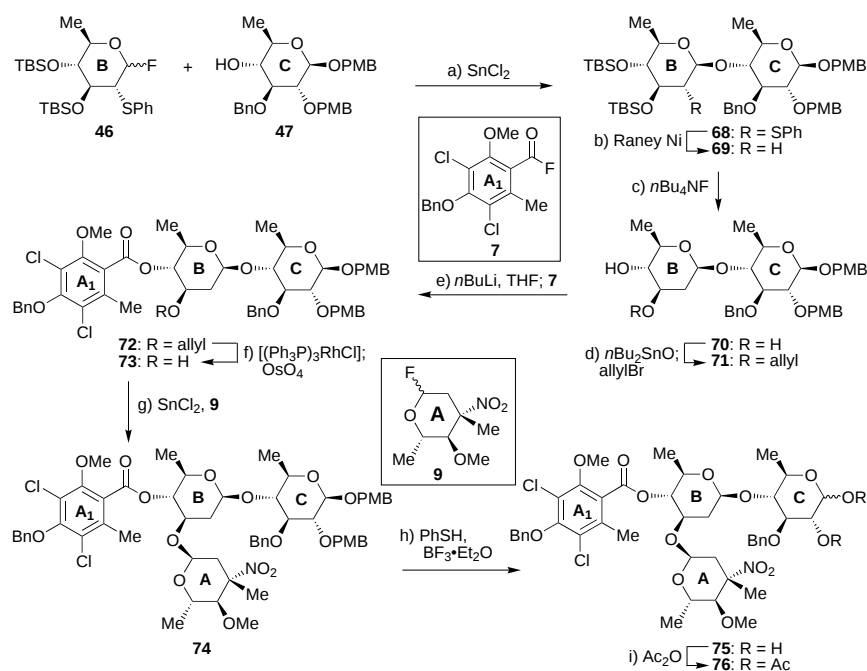
Scheme 8. Construction of A 1 B(A)C fragment 76 . a) 1.0 equiv 46 , 0.9 equiv 47 , 1.8 equiv SnCl 2 , 4 Å MS, CH 2 Cl 2 /Et 2 O/Me 2 S 1:1:1, -10^{\circ} C, 3 h, 71%; b) ca. 1.0 equiv Raney Ni ( w/w ), EtOH/THF 1:1, reflux, 8 h; c) 2.2 equiv n Bu 4 NF, THF, 25 ^{\circ} C, 2 h, 78% over two steps; d) 1.1 equiv n Bu 2 SnO, toluene, reflux, 3 h; 1.5 equiv allyl bromide, 0.2 equiv n Bu 4 NI, 25 \rightarrow 110 ^{\circ} C, 3 h, 93%; e) 1.1 equiv n BuLi, THF, -78 \rightarrow 0^{\circ} C, 1 h; 1.2 equiv 7 , THF, 0 \rightarrow 25 ^{\circ} C, 4 h, 99%; f) i) 1.5 equiv DABCO, 0.05 equiv [(Ph 3 P) 3 RhCl], EtOH/H 2 O 10:1, reflux, 2 h; ii) 1.1 equiv NMO, 0.05 equiv OsO 4 , acetone/H 2 O 10:1, 25 ^{\circ} C, 3 h, 81%; g) 1.7 equiv 9 , 1.6 equiv SnCl 2 , CH 2 Cl 2 /Et 2 O 1:1, 0 \rightarrow 25 ^{\circ} C, 1 h, 77%; h) 8.0 equiv PhSH, 4.0 equiv BF 3 ·Et 2 O, CH 2 Cl 2 , -35^{\circ} C, 2 h, 83%; i) 2.5 equiv Ac 2 O, 4.0 equiv Et 3 N, 0.2 equiv 4-DMAP, CH 2 Cl 2 , 0 \rightarrow 25 ^{\circ} C, 1 h, 97%. DABCO = 1,4-diazabicyclo[2.2.2]octane.
