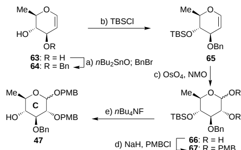
Scheme 7. Synthesis of carbohydrate building block C ( 47 ). a) 1.1 equiv n Bu 2 SnO, toluene, reflux, 3 h; 1.5 equiv BnBr, 0.2 equiv n Bu 4 NI, 25 \rightarrow 110 ^{\circ} C, 3 h, 83%; b) 1.5 equiv TBSCl, 2.5 equiv imidazole, CH 2 Cl 2 , 0 \rightarrow 25 ^{\circ} C, 3 h, 93%; c) 1.1 equiv NMO, 0.05 equiv OsO 4 , acetone/H 2 O 10:1, 25 ^{\circ} C, 8 h, 97%; d) 2.4 equiv NaH, 3.0 equiv PMBCl, 0.2 equiv n Bu 4 NI, DMF, 0 \rightarrow 25 ^{\circ} C, 3 h, 95%; e) 1.1 equiv n Bu 4 NF, THF, 25 ^{\circ} C, 1 h, 95%, \alpha : \beta ca. 1:1.
