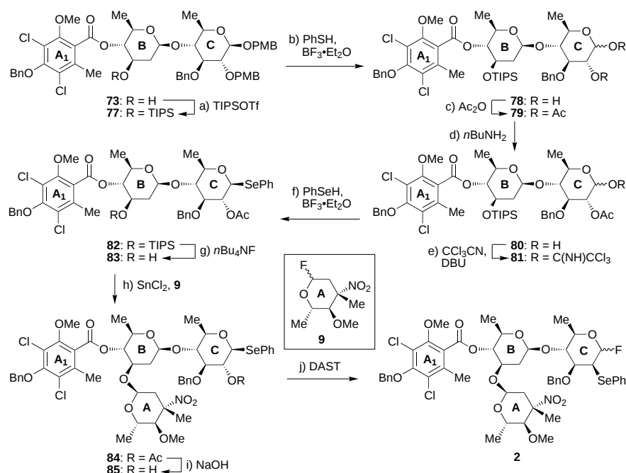
Scheme 9. Construction of \text{A}_1\text{B(A)C} fragment 2 . a) 1.2 equiv TIPSOTf, 1.5 equiv 2,6-lutidine, \text{CH}_2\text{Cl}_2 , 0 \rightarrow 25^\circ\text{C} , 1 h, 93 %; b) 8.0 equiv PhSH, 4.0 equiv \text{BF}_3 \cdot \text{Et}_2\text{O} , \text{CH}_2\text{Cl}_2 , -35^\circ\text{C} , 2 h, 83 %; c) 2.5 equiv \text{Ac}_2\text{O} , 4.0 equiv \text{Et}_3\text{N} , 0.2 equiv 4-DMAP, \text{CH}_2\text{Cl}_2 , 0 \rightarrow 25^\circ\text{C} , 1 h, 98 %; d) 1.3 equiv n\text{BuNH}_2 , THF, 25^\circ\text{C} , 5 h, 91 %; e) 5.0 equiv \text{CCl}_3\text{CN} , 0.05 equiv DBU, \text{CH}_2\text{Cl}_2 , 0^\circ\text{C} , 0.5 h; f) ca. 2.0 equiv PhSeH, 0.2 equiv \text{BF}_3 \cdot \text{Et}_2\text{O} , \text{CH}_2\text{Cl}_2 , -78^\circ\text{C} , 1 h, 78 % over two steps, \alpha:\beta ca. 1:9; g) 1.2 equiv n\text{Bu}_4\text{NF} , THF, 25^\circ\text{C} , 1 h, 91 %; h) 2.0 equiv 9 , 1.2 equiv \text{SnCl}_2 , \text{CH}_2\text{Cl}_2/\text{Et}_2\text{O} 1:1, 0 \rightarrow 25^\circ\text{C} , 1 h, 80 %; i) 0.3 equiv NaOH, \text{MeOH}/\text{Et}_2\text{O} 1:1, 25^\circ\text{C} , 1 h, 91 %; j) 1.5 equiv DAST, \text{CH}_2\text{Cl}_2 , 0^\circ\text{C} , 20 min, 100 %, \alpha:\beta ca. 8:1. DBU = 1,8-diazabicyclo[5.4.0]undec-7-ene.
